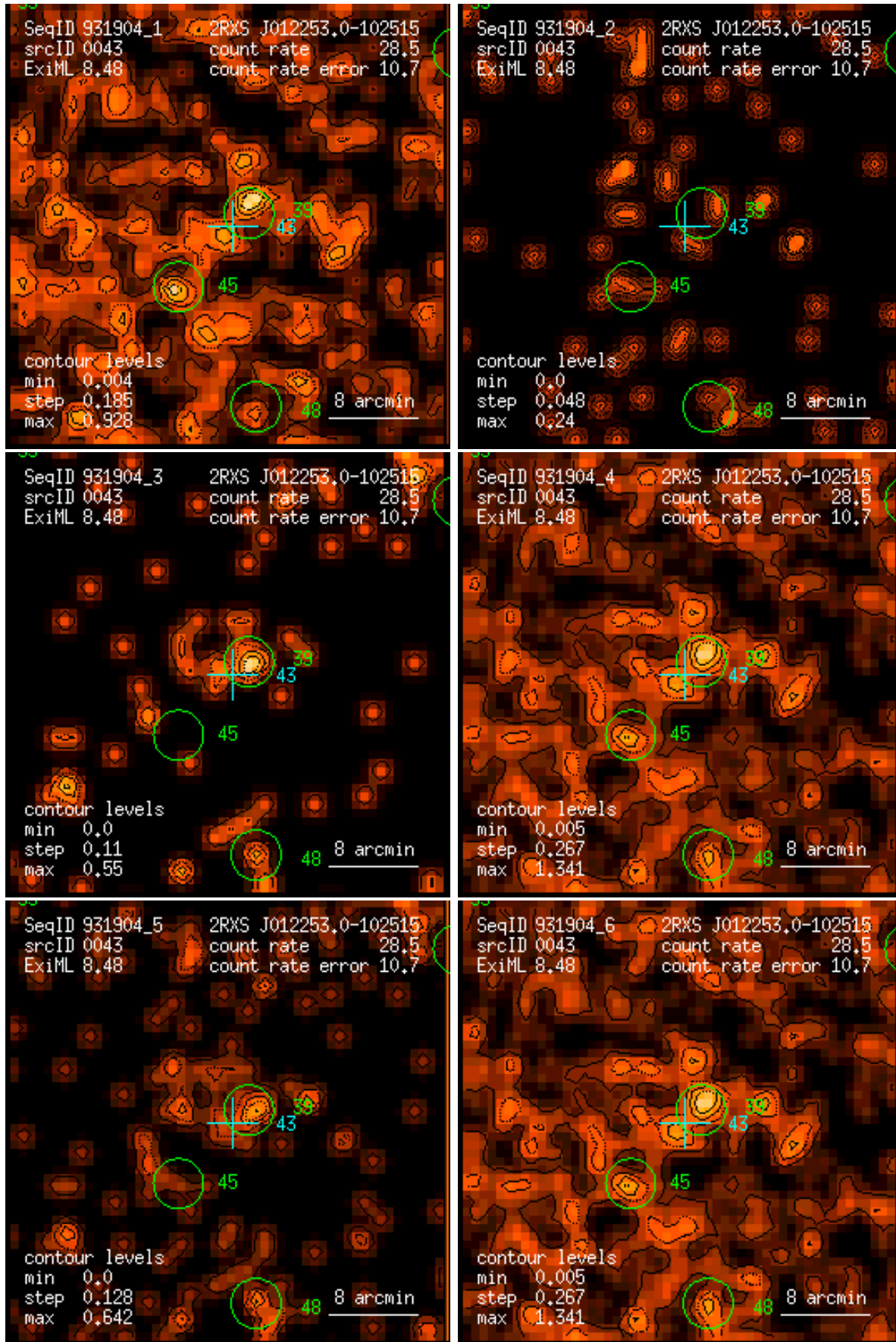
Figure 43: RASS 931904: detection 0043: band rate images, Gaussian filter: (1) PSPC channels 11 – 41, (2) 52 – 90, (3) 91 – 201, (4) 11 – 235, (5) 52 – 201, (6) 11 – 201. Broad band rates in counts/ks. Band rate contour levels in counts/ks/arcmin 2 .
