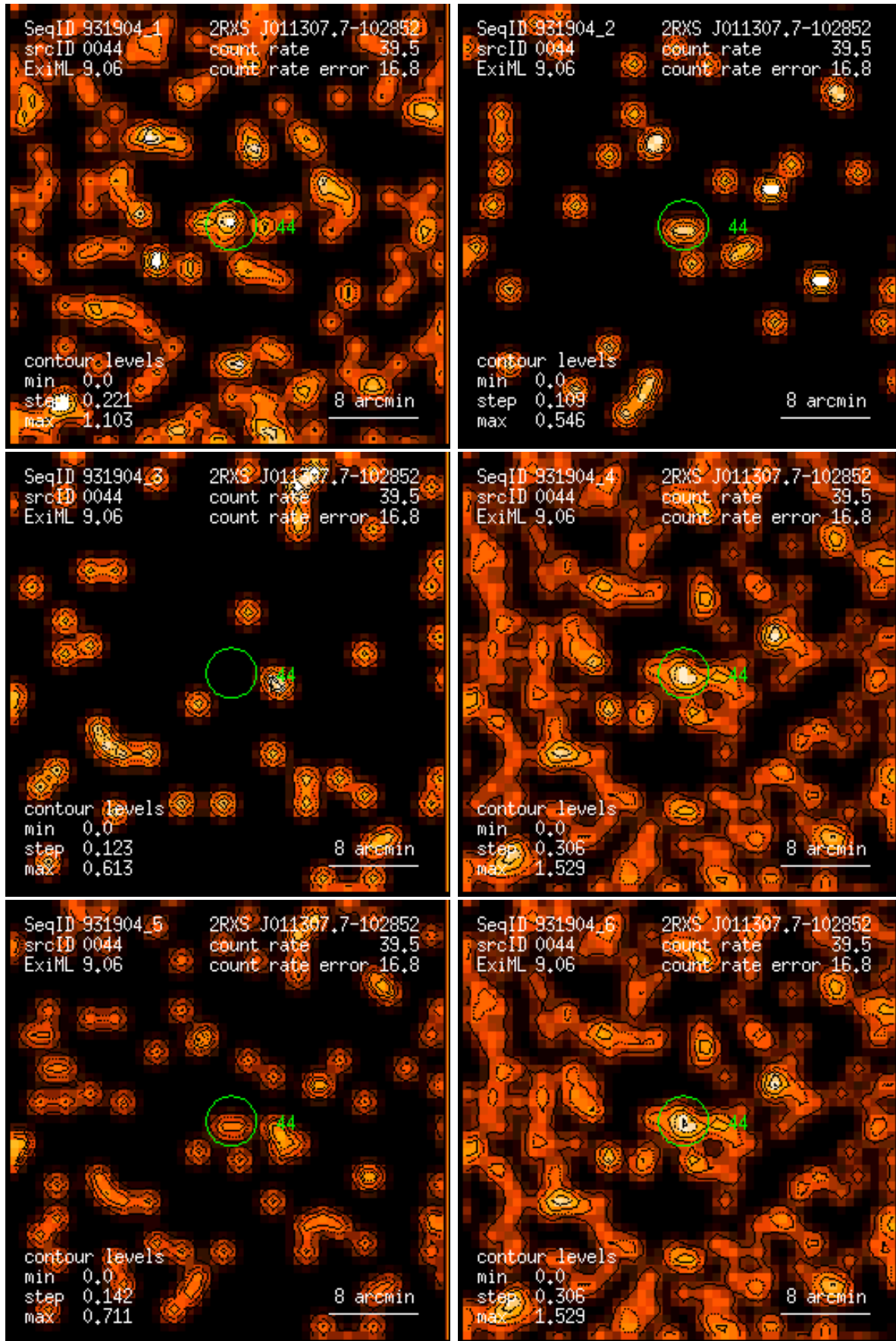
Figure 44: RASS 931904: detection 0044: band rate images, Gaussian filter: (1) PSPC channels 11 – 41, (2) 52 – 90, (3) 91 – 201, (4) 11 – 235, (5) 52 – 201, (6) 11 – 201. Broad band rates in counts/ks. Band rate contour levels in counts/ks/arcmin 2 .
