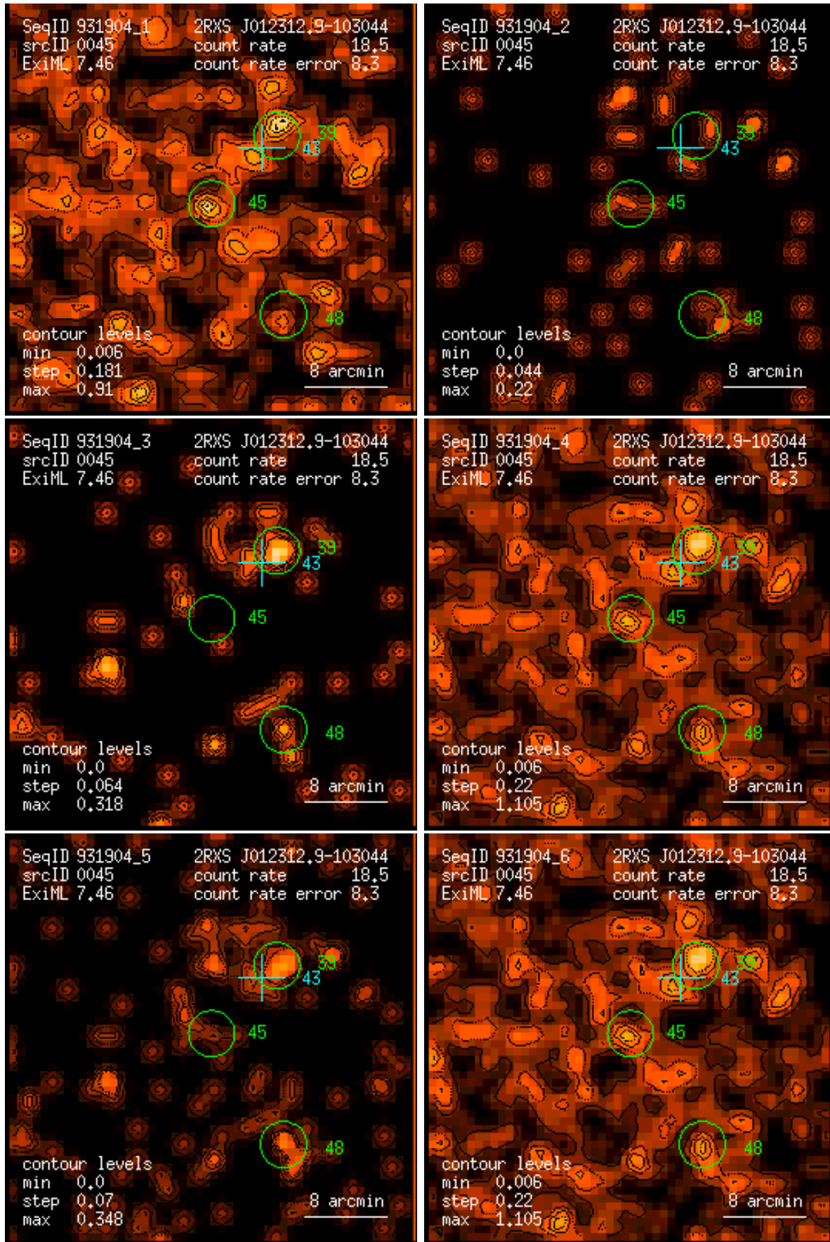
Figure 45: RASS 931904: detection 0045: band rate images, Gaussian filter: (1) PSPC channels 11 – 41, (2) 52 – 90, (3) 91 – 201, (4) 11 – 235, (5) 52 – 201, (6) 11 – 201. Broad band rates in counts/ks. Band rate contour levels in counts/ks/arcmin 2 .
