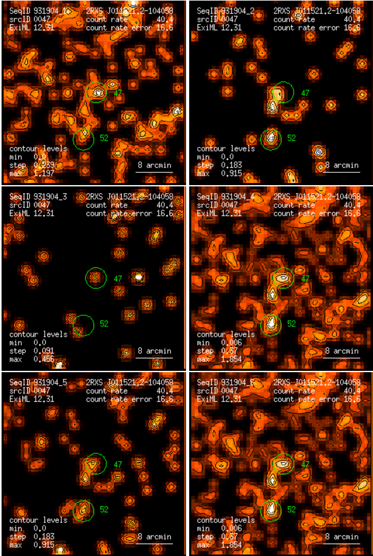
Figure 47: RASS 931904: detection 0047: band rate images, Gaussian filter: (1) PSPC channels 11 – 41, (2) 52 – 90, (3) 91 – 201, (4) 11 – 235, (5) 52 – 201, (6) 11 – 201. Broad band rates in counts/ks. Band rate contour levels in counts/ks/arcmin 2 .
