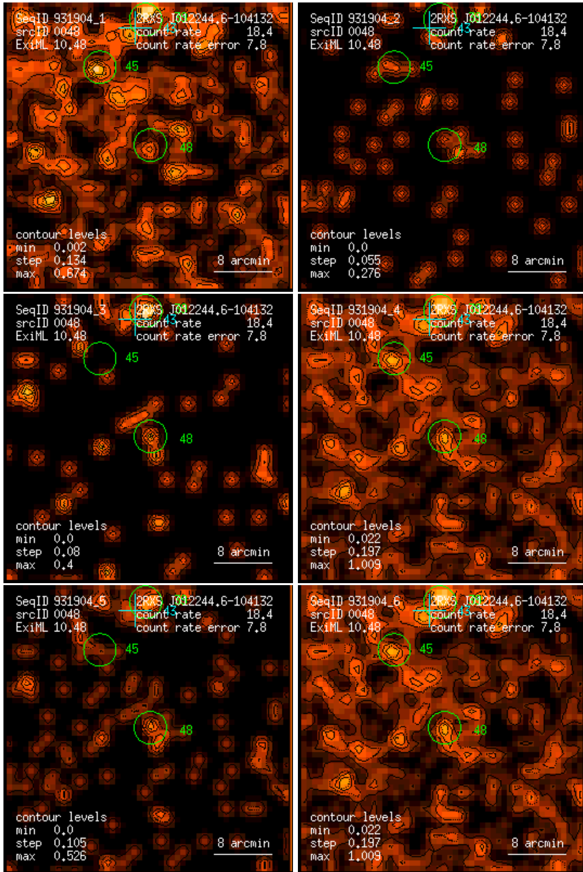
Figure 48: RASS 931904: detection 0048: band rate images, Gaussian filter: (1) PSPC channels 11 – 41, (2) 52 – 90, (3) 91 – 201, (4) 11 – 235, (5) 52 – 201, (6) 11 – 201. Broad band rates in counts/ks. Band rate contour levels in counts/ks/arcmin 2 .
