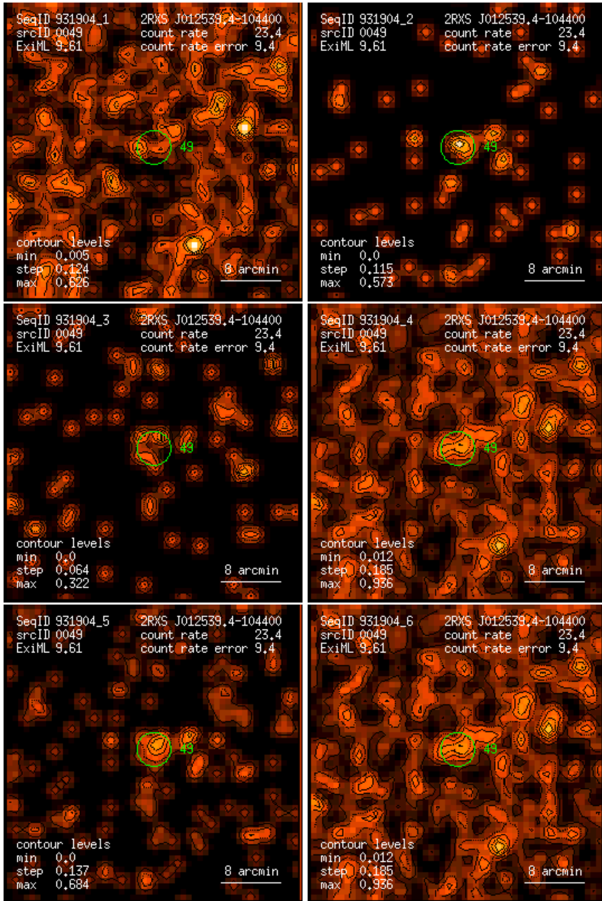
Figure 49: RASS 931904: detection 0049: band rate images, Gaussian filter: (1) PSPC channels 11 – 41, (2) 52 – 90, (3) 91 – 201, (4) 11 – 235, (5) 52 – 201, (6) 11 – 201. Broad band rates in counts/ks. Band rate contour levels in counts/ks/arcmin 2 .
