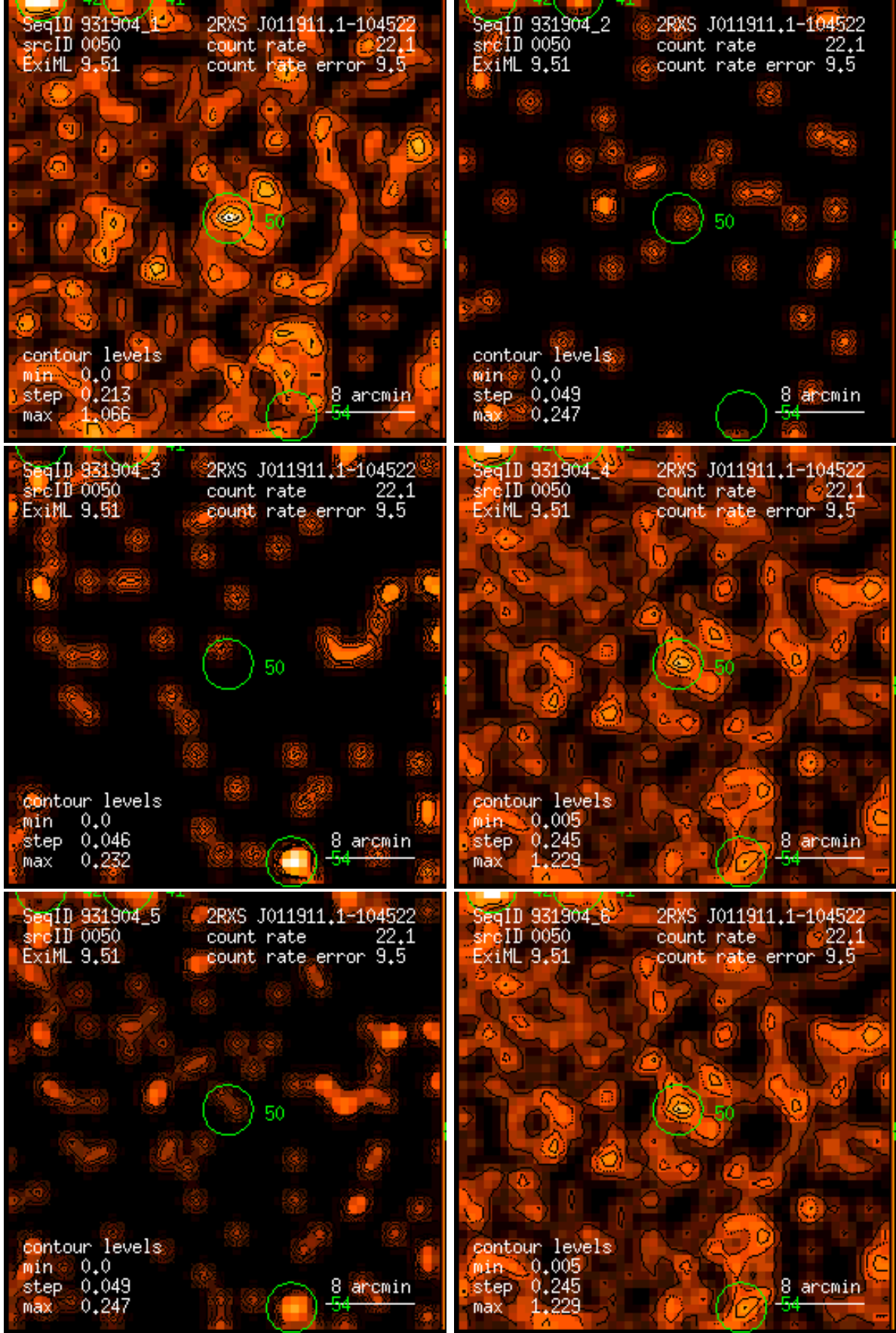
Figure 50: RASS 931904: detection 0050: band rate images, Gaussian filter: (1) PSPC channels 11 – 41, (2) 52 – 90, (3) 91 – 201, (4) 11 – 235, (5) 52 – 201, (6) 11 – 201. Broad band rates in counts/ks. Band rate contour levels in counts/ks/arcmin 2 .
