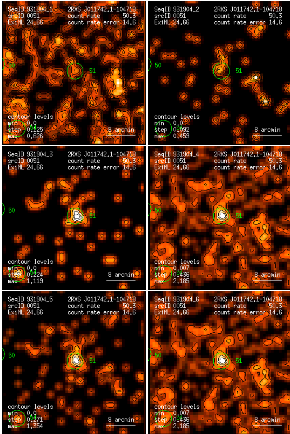
Figure 51: RASS 931904: detection 0051: band rate images, Gaussian filter: (1) PSPC channels 11 – 41, (2) 52 – 90, (3) 91 – 201, (4) 11 – 235, (5) 52 – 201, (6) 11 – 201. Broad band rates in counts/ks. Band rate contour levels in counts/ks/arcmin 2 .
