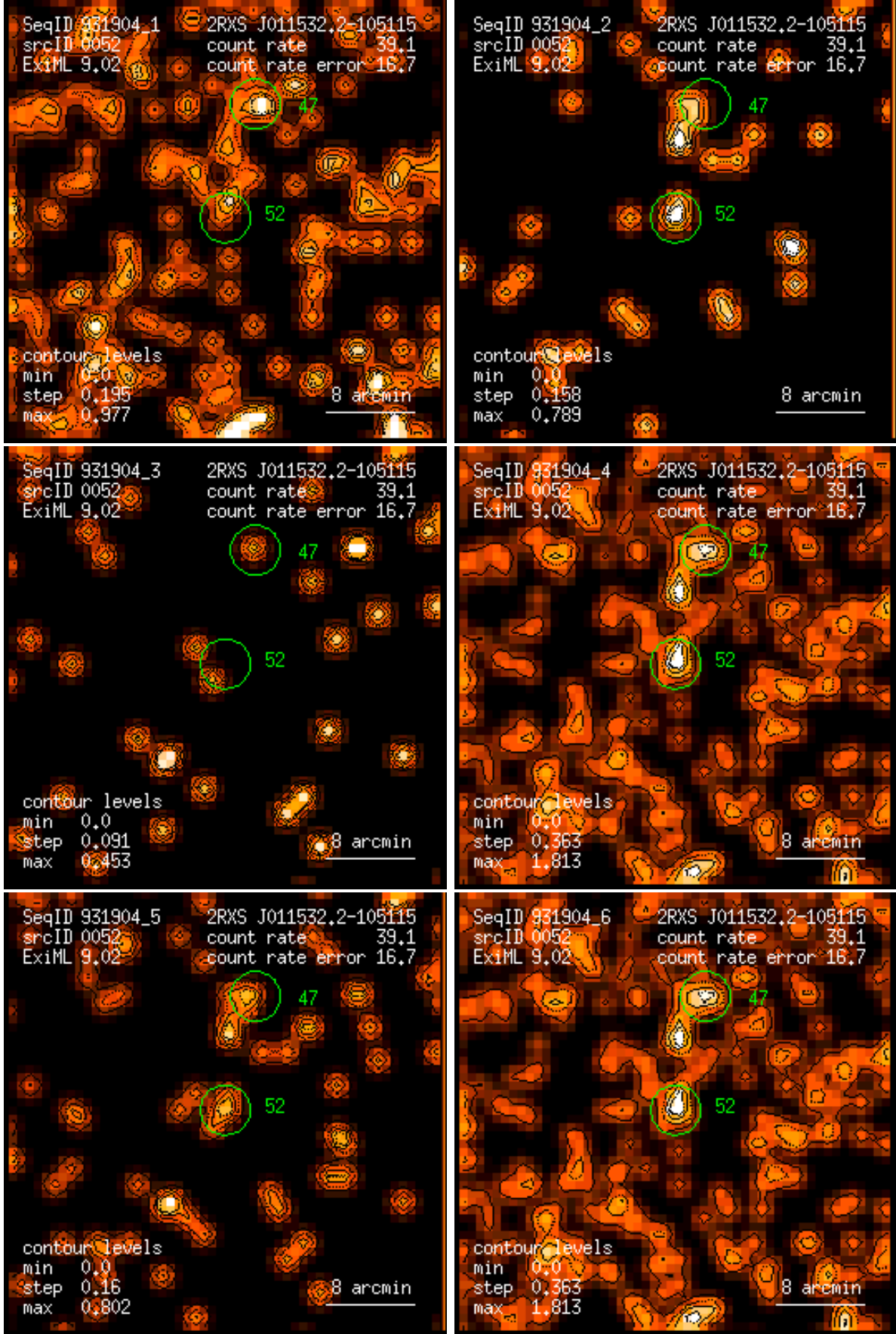
Figure 52: RASS 931904: detection 0052: band rate images, Gaussian filter: (1) PSPC channels 11 – 41, (2) 52 – 90, (3) 91 – 201, (4) 11 – 235, (5) 52 – 201, (6) 11 – 201. Broad band rates in counts/ks. Band rate contour levels in counts/ks/arcmin 2 .
