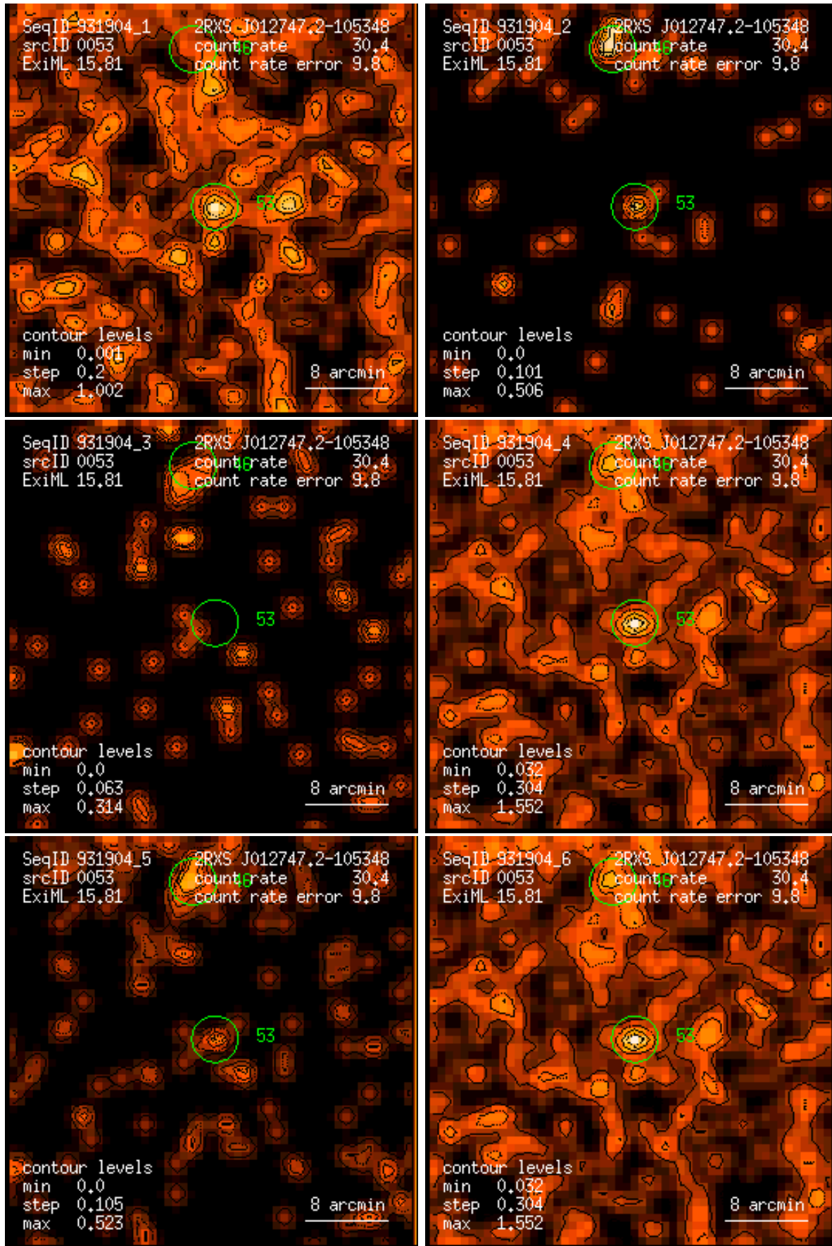
Figure 53: RASS 931904: detection 0053: band rate images, Gaussian filter: (1) PSPC channels 11 – 41, (2) 52 – 90, (3) 91 – 201, (4) 11 – 235, (5) 52 – 201, (6) 11 – 201. Broad band rates in counts/ks. Band rate contour levels in counts/ks/arcmin 2 .
