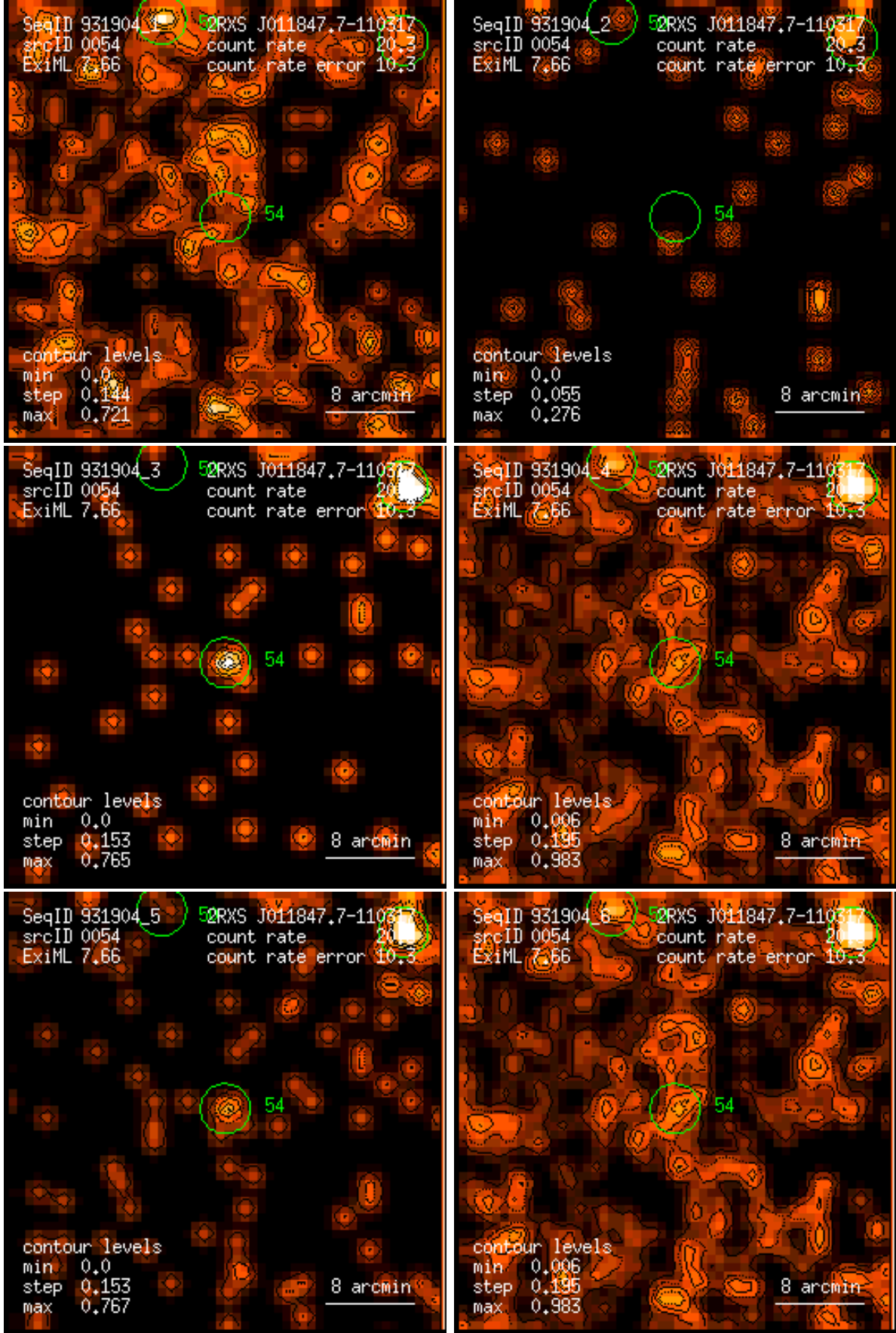
Figure 54: RASS 931904: detection 0054: band rate images, Gaussian filter: (1) PSPC channels 11 – 41, (2) 52 – 90, (3) 91 – 201, (4) 11 – 235, (5) 52 – 201, (6) 11 – 201. Broad band rates in counts/ks. Band rate contour levels in counts/ks/arcmin 2 .
