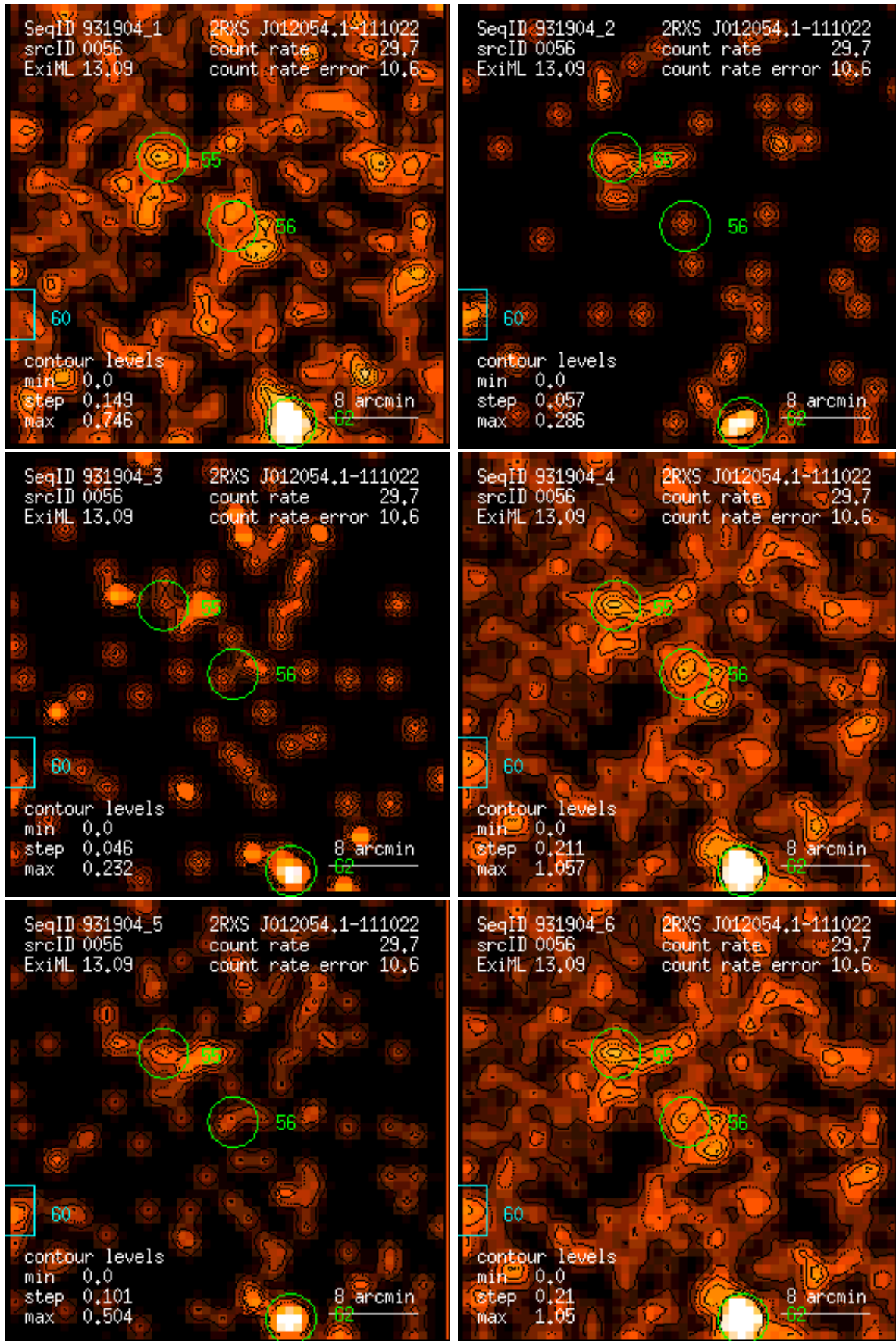
Figure 56: RASS 931904: detection 0056: band rate images, Gaussian filter: (1) PSPC channels 11 – 41, (2) 52 – 90, (3) 91 – 201, (4) 11 – 235, (5) 52 – 201, (6) 11 – 201. Broad band rates in counts/ks. Band rate contour levels in counts/ks/arcmin 2 .
