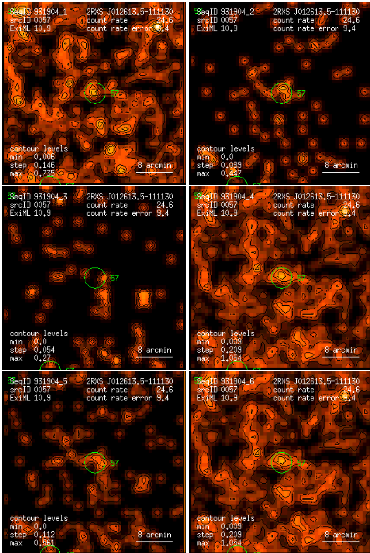
Figure 57: RASS 931904: detection 0057: band rate images, Gaussian filter: (1) PSPC channels 11 – 41, (2) 52 – 90, (3) 91 – 201, (4) 11 – 235, (5) 52 – 201, (6) 11 – 201. Broad band rates in counts/ks. Band rate contour levels in counts/ks/arcmin 2 .
