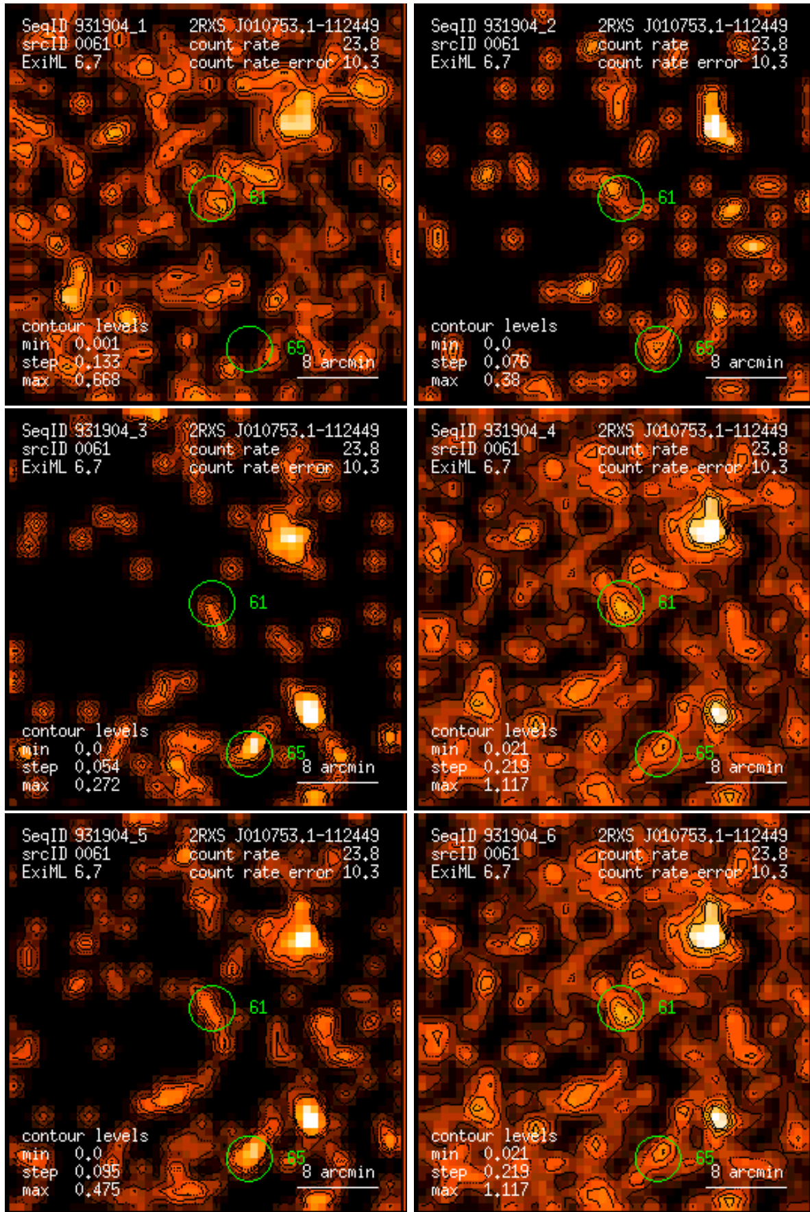
Figure 61: RASS 931904: detection 0061: band rate images, Gaussian filter: (1) PSPC channels 11 – 41, (2) 52 – 90, (3) 91 – 201, (4) 11 – 235, (5) 52 – 201, (6) 11 – 201. Broad band rates in counts/ks. Band rate contour levels in counts/ks/arcmin 2 .
