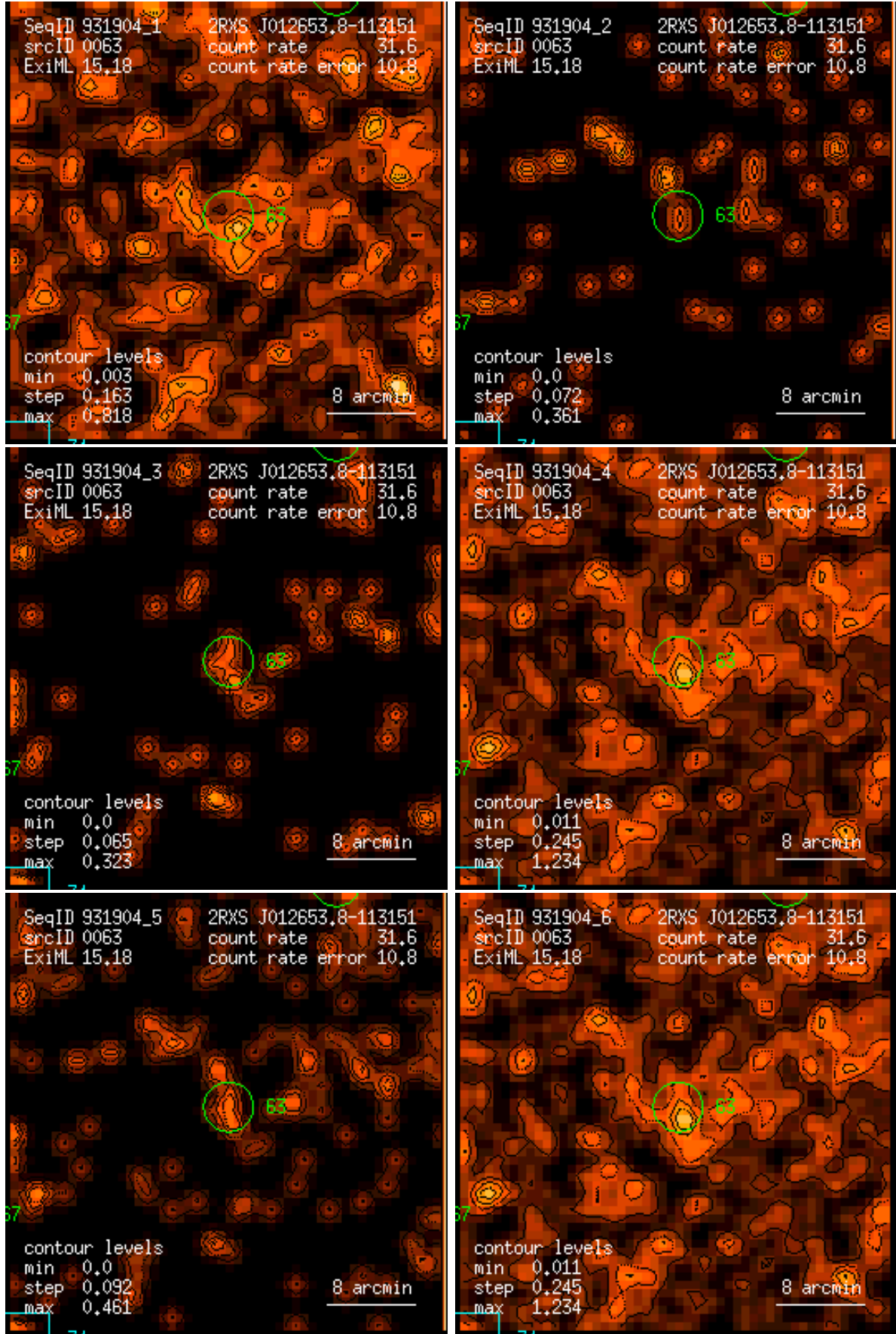
Figure 63: RASS 931904: detection 0063: band rate images, Gaussian filter: (1) PSPC channels 11 – 41, (2) 52 – 90, (3) 91 – 201, (4) 11 – 235, (5) 52 – 201, (6) 11 – 201. Broad band rates in counts/ks. Band rate contour levels in counts/ks/arcmin 2 .
