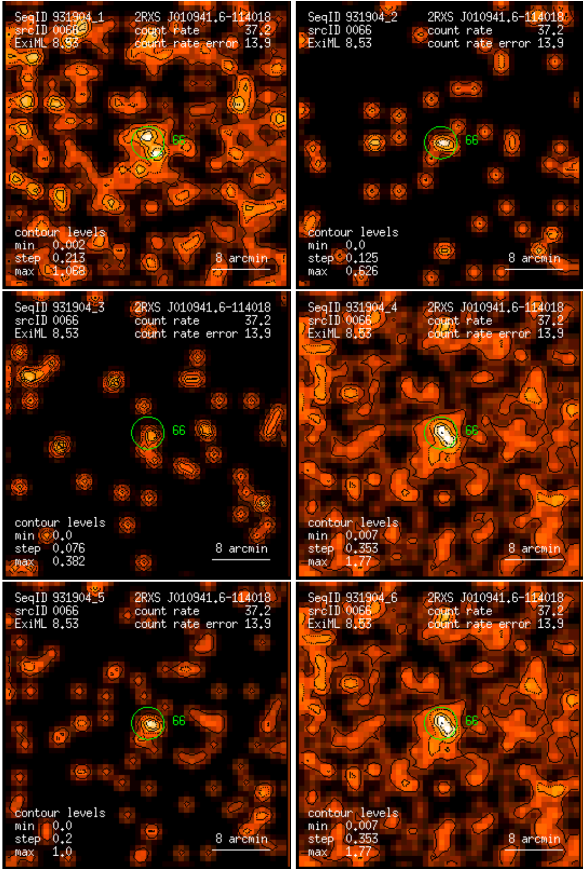
Figure 66: RASS 931904: detection 0066: band rate images, Gaussian filter: (1) PSPC channels 11 – 41, (2) 52 – 90, (3) 91 – 201, (4) 11 – 235, (5) 52 – 201, (6) 11 – 201. Broad band rates in counts/ks. Band rate contour levels in counts/ks/arcmin 2 .
