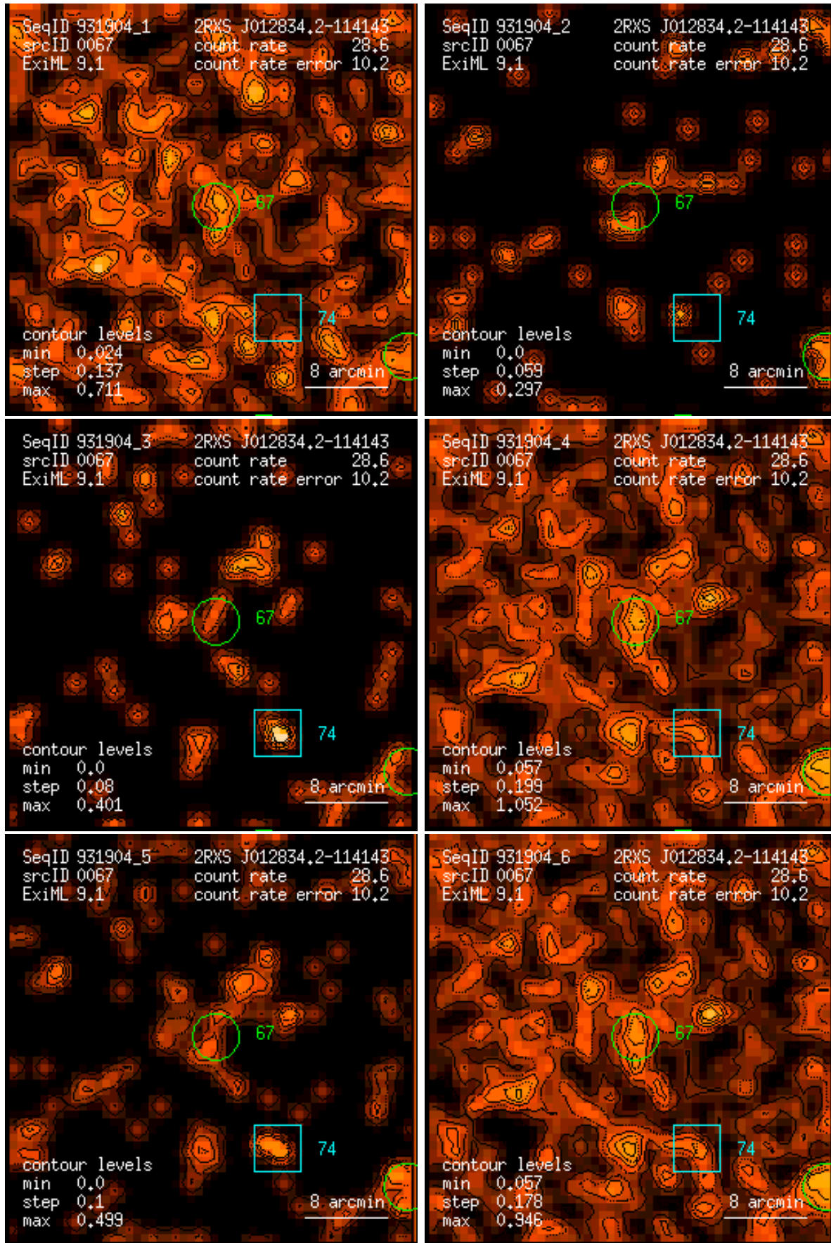
Figure 67: RASS 931904: detection 0067: band rate images, Gaussian filter: (1) PSPC channels 11 – 41, (2) 52 – 90, (3) 91 – 201, (4) 11 – 235, (5) 52 – 201, (6) 11 – 201. Broad band rates in counts/ks. Band rate contour levels in counts/ks/arcmin 2 .
