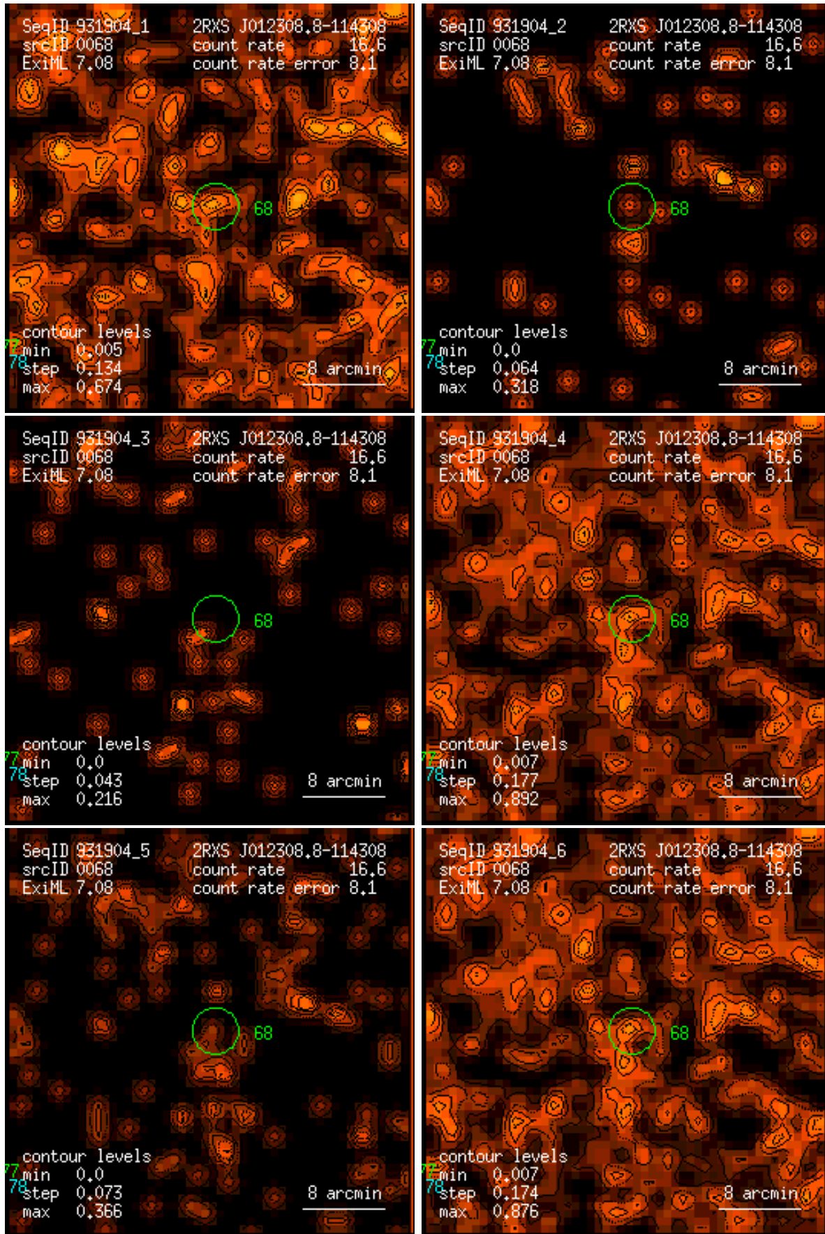
Figure 68: RASS 931904: detection 0068: band rate images, Gaussian filter: (1) PSPC channels 11 – 41, (2) 52 – 90, (3) 91 – 201, (4) 11 – 235, (5) 52 – 201, (6) 11 – 201. Broad band rates in counts/ks. Band rate contour levels in counts/ks/arcmin 2 .
