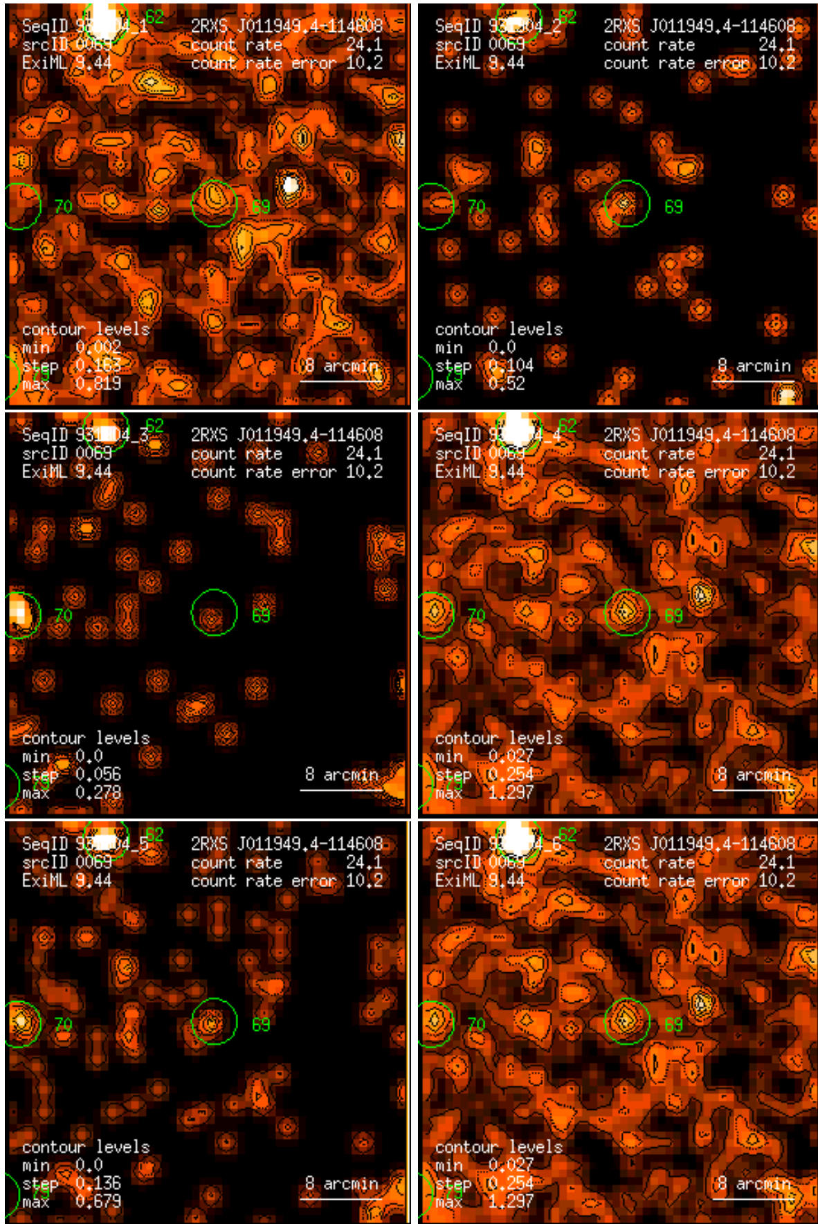
Figure 69: RASS 931904: detection 0069: band rate images, Gaussian filter: (1) PSPC channels 11 – 41, (2) 52 – 90, (3) 91 – 201, (4) 11 – 235, (5) 52 – 201, (6) 11 – 201. Broad band rates in counts/ks. Band rate contour levels in counts/ks/arcmin 2 .
