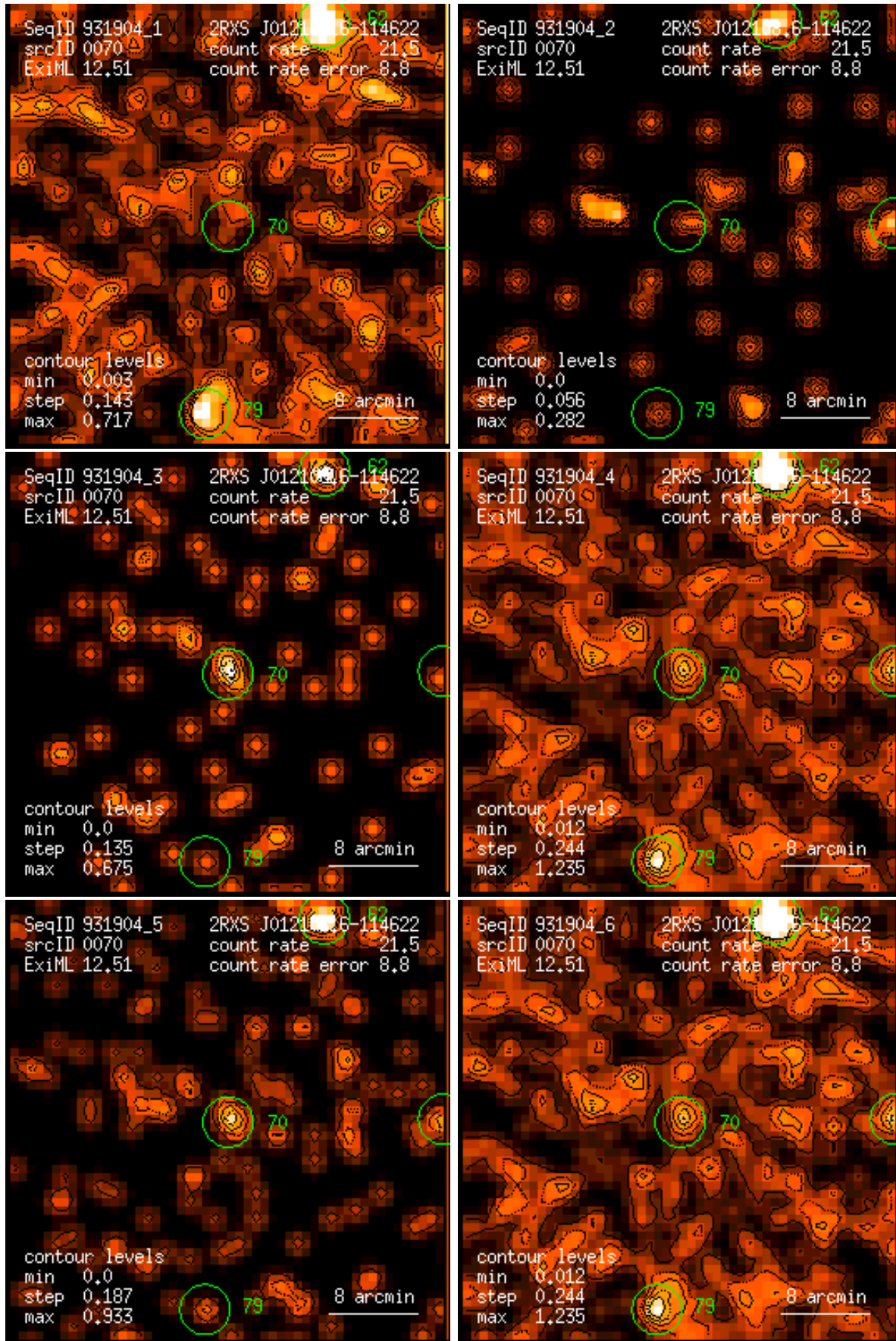
Figure 70: RASS 931904: detection 0070: band rate images, Gaussian filter: (1) PSPC channels 11 – 41, (2) 52 – 90, (3) 91 – 201, (4) 11 – 235, (5) 52 – 201, (6) 11 – 201. Broad band rates in counts/ks. Band rate contour levels in counts/ks/arcmin 2 .
