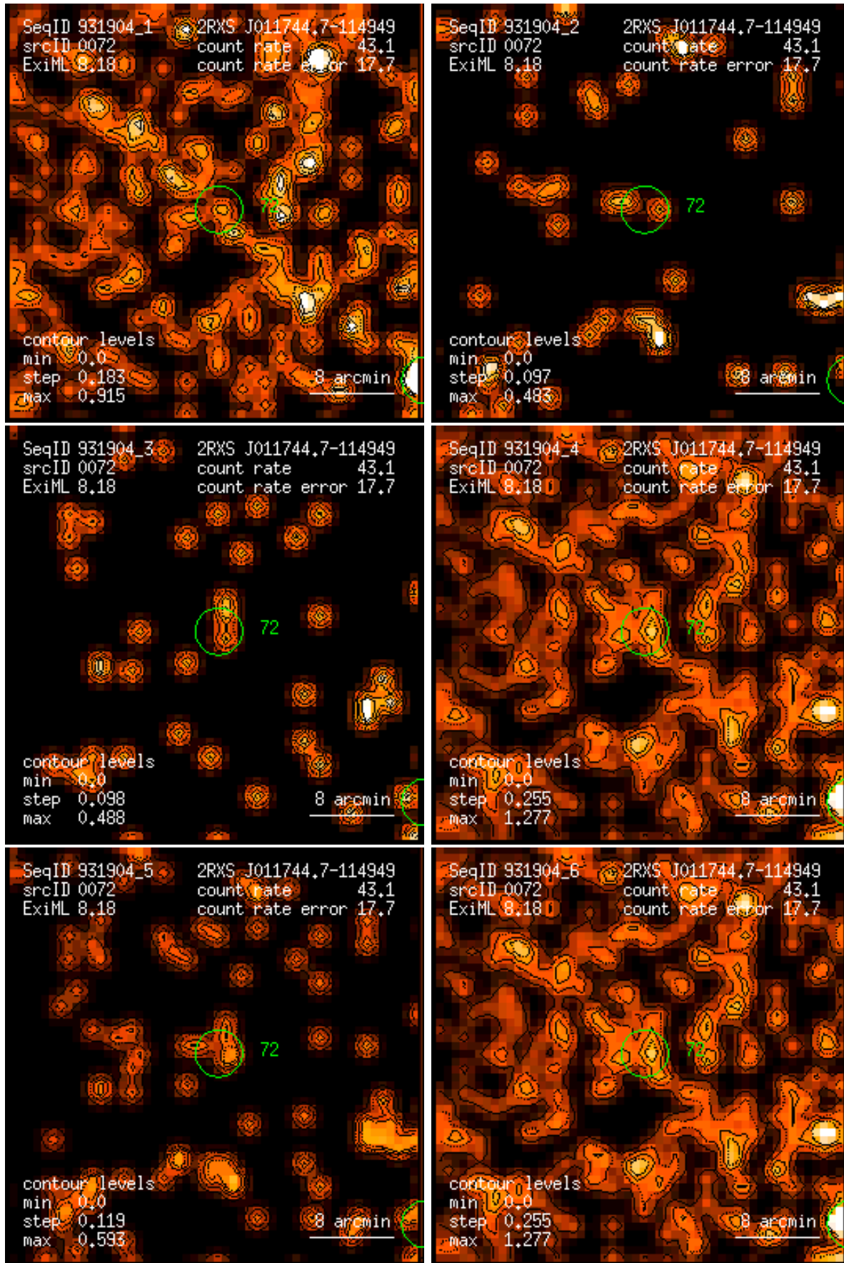
Figure 72: RASS 931904: detection 0072: band rate images, Gaussian filter: (1) PSPC channels 11 – 41, (2) 52 – 90, (3) 91 – 201, (4) 11 – 235, (5) 52 – 201, (6) 11 – 201. Broad band rates in counts/ks. Band rate contour levels in counts/ks/arcmin 2 .
