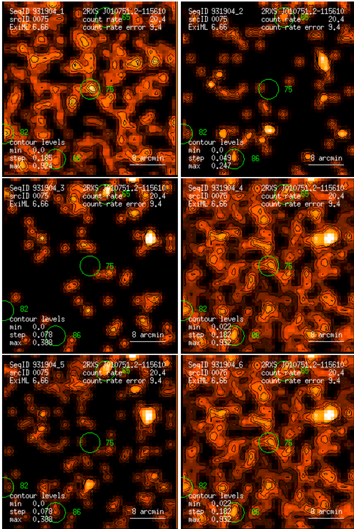
Figure 75: RASS 931904: detection 0075: band rate images, Gaussian filter: (1) PSPC channels 11 – 41, (2) 52 – 90, (3) 91 – 201, (4) 11 – 235, (5) 52 – 201, (6) 11 – 201. Broad band rates in counts/ks. Band rate contour levels in counts/ks/arcmin 2 .
