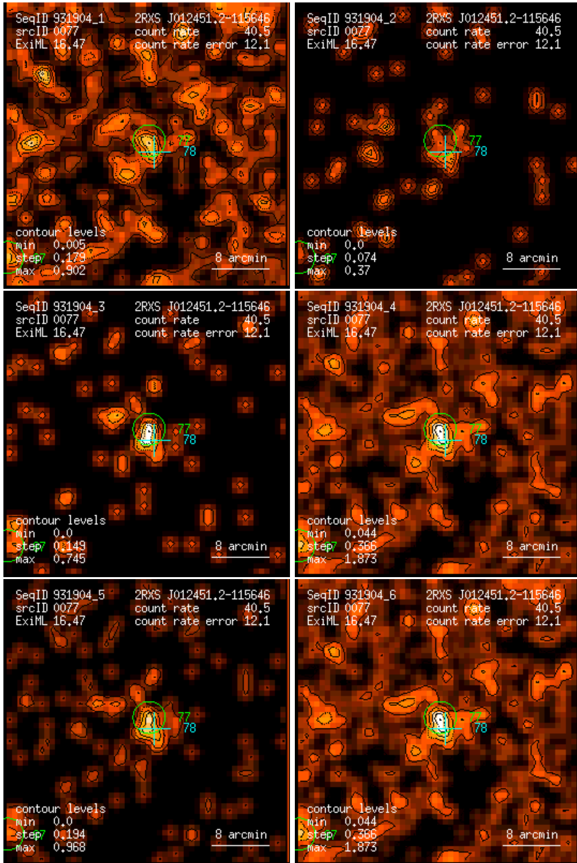
Figure 77: RASS 931904: detection 0077: band rate images, Gaussian filter: (1) PSPC channels 11 – 41, (2) 52 – 90, (3) 91 – 201, (4) 11 – 235, (5) 52 – 201, (6) 11 – 201. Broad band rates in counts/ks. Band rate contour levels in counts/ks/arcmin 2 .
