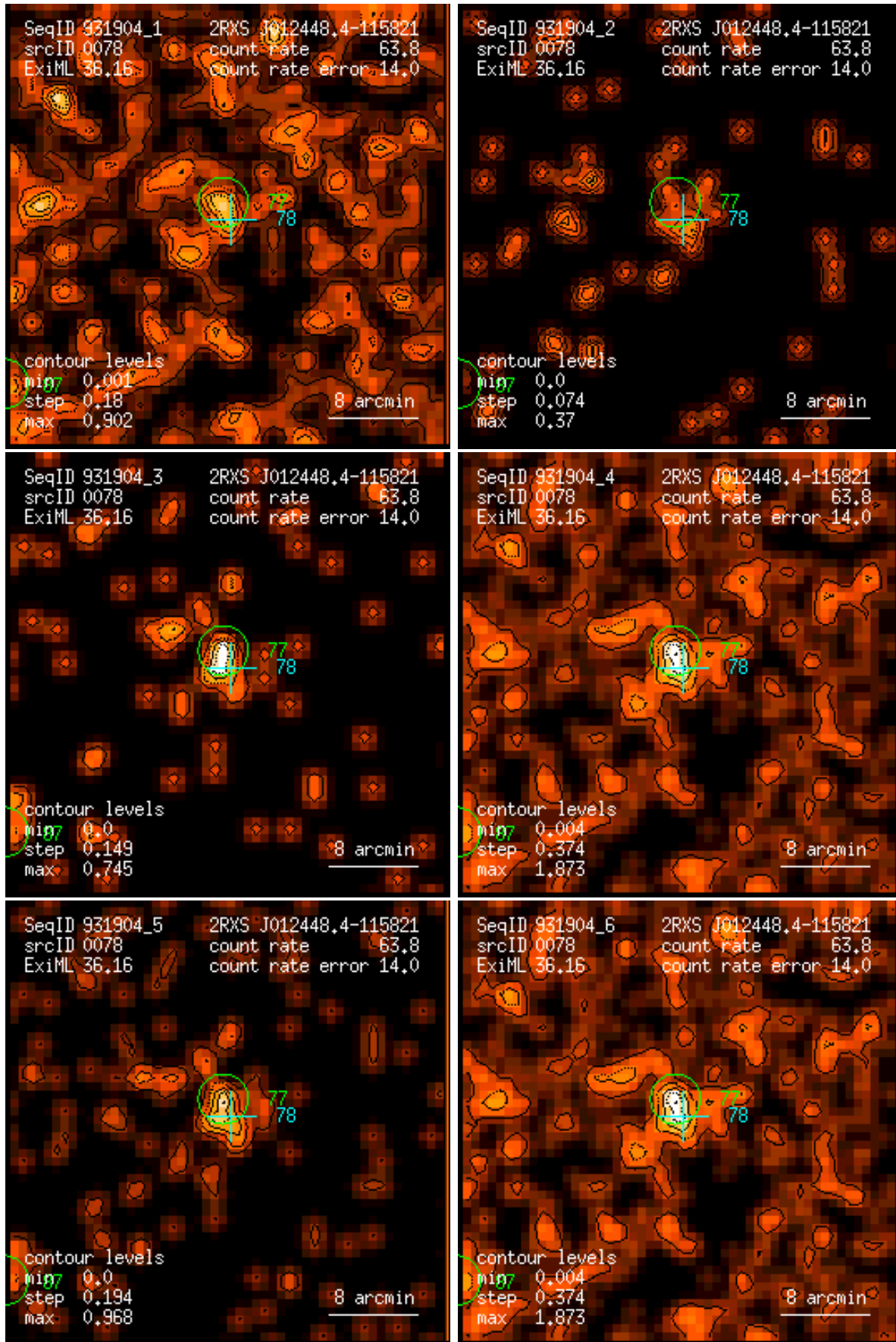
Figure 78: RASS 931904: detection 0078: band rate images, Gaussian filter: (1) PSPC channels 11 – 41, (2) 52 – 90, (3) 91 – 201, (4) 11 – 235, (5) 52 – 201, (6) 11 – 201. Broad band rates in counts/ks. Band rate contour levels in counts/ks/arcmin 2 .
