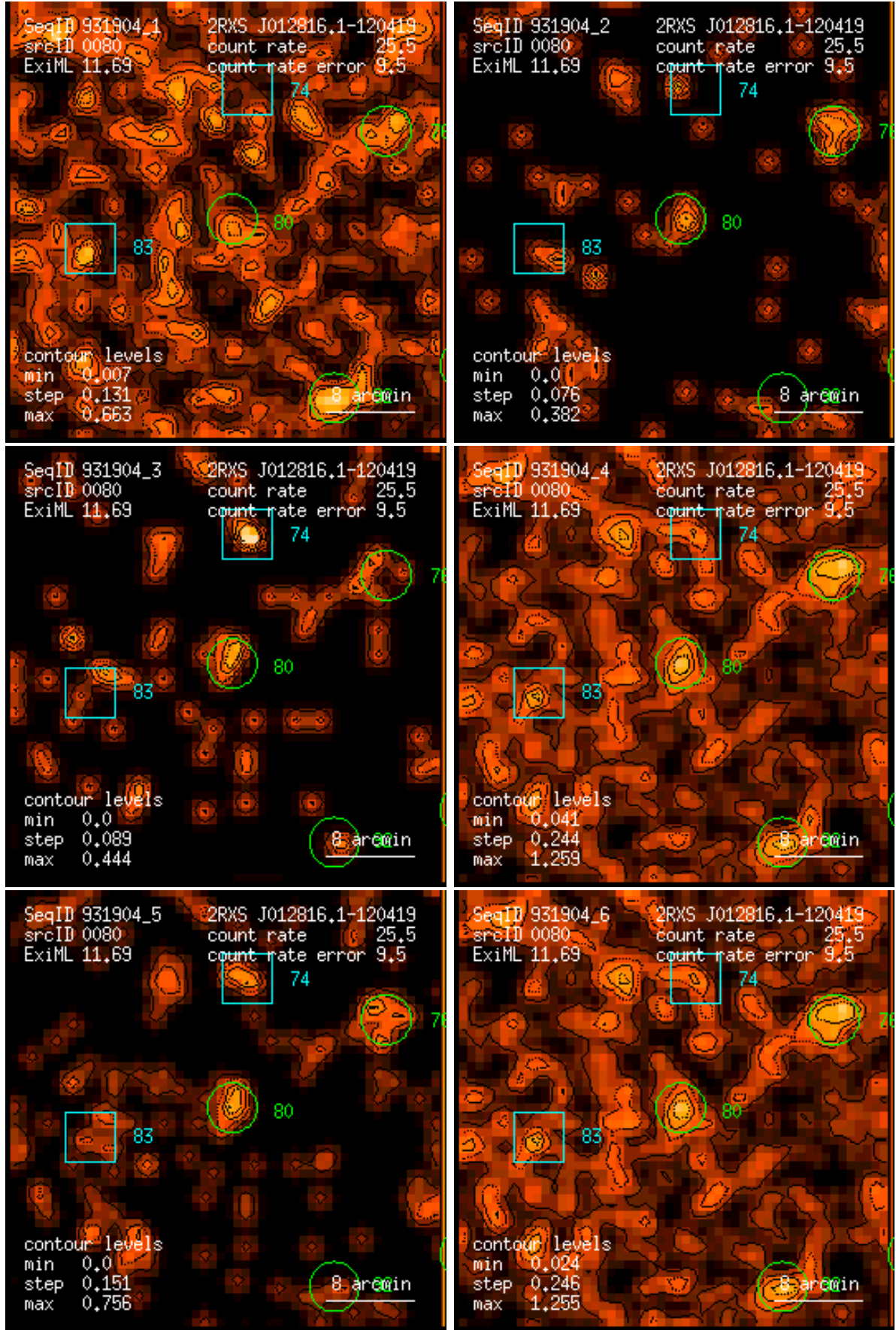
Figure 80: RASS 931904: detection 0080: band rate images, Gaussian filter: (1) PSPC channels 11 – 41, (2) 52 – 90, (3) 91 – 201, (4) 11 – 235, (5) 52 – 201, (6) 11 – 201. Broad band rates in counts/ks. Band rate contour levels in counts/ks/arcmin 2 .
