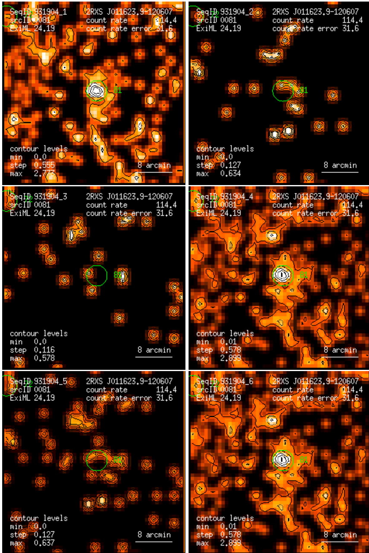
Figure 81: RASS 931904: detection 0081: band rate images, Gaussian filter: (1) PSPC channels 11 – 41, (2) 52 – 90, (3) 91 – 201, (4) 11 – 235, (5) 52 – 201, (6) 11 – 201. Broad band rates in counts/ks. Band rate contour levels in counts/ks/arcmin 2 .
