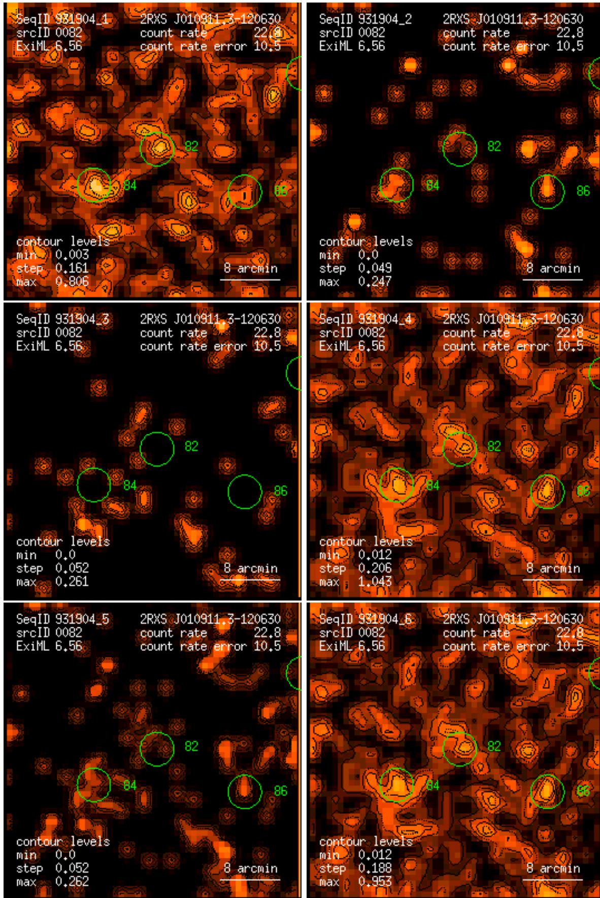
Figure 82: RASS 931904: detection 0082: band rate images, Gaussian filter: (1) PSPC channels 11 – 41, (2) 52 – 90, (3) 91 – 201, (4) 11 – 235, (5) 52 – 201, (6) 11 – 201. Broad band rates in counts/ks. Band rate contour levels in counts/ks/arcmin 2 .
