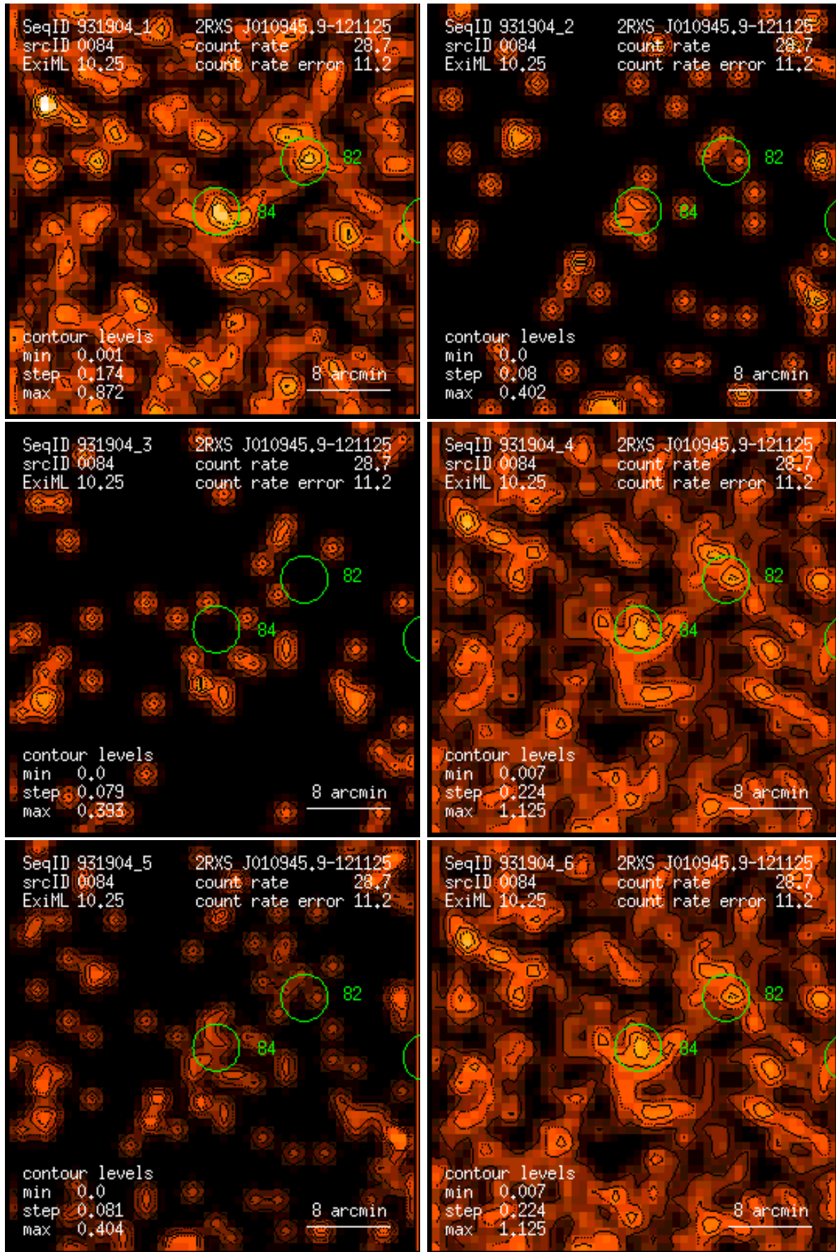
Figure 84: RASS 931904: detection 0084: band rate images, Gaussian filter: (1) PSPC channels 11 – 41, (2) 52 – 90, (3) 91 – 201, (4) 11 – 235, (5) 52 – 201, (6) 11 – 201. Broad band rates in counts/ks. Band rate contour levels in counts/ks/arcmin 2 .
