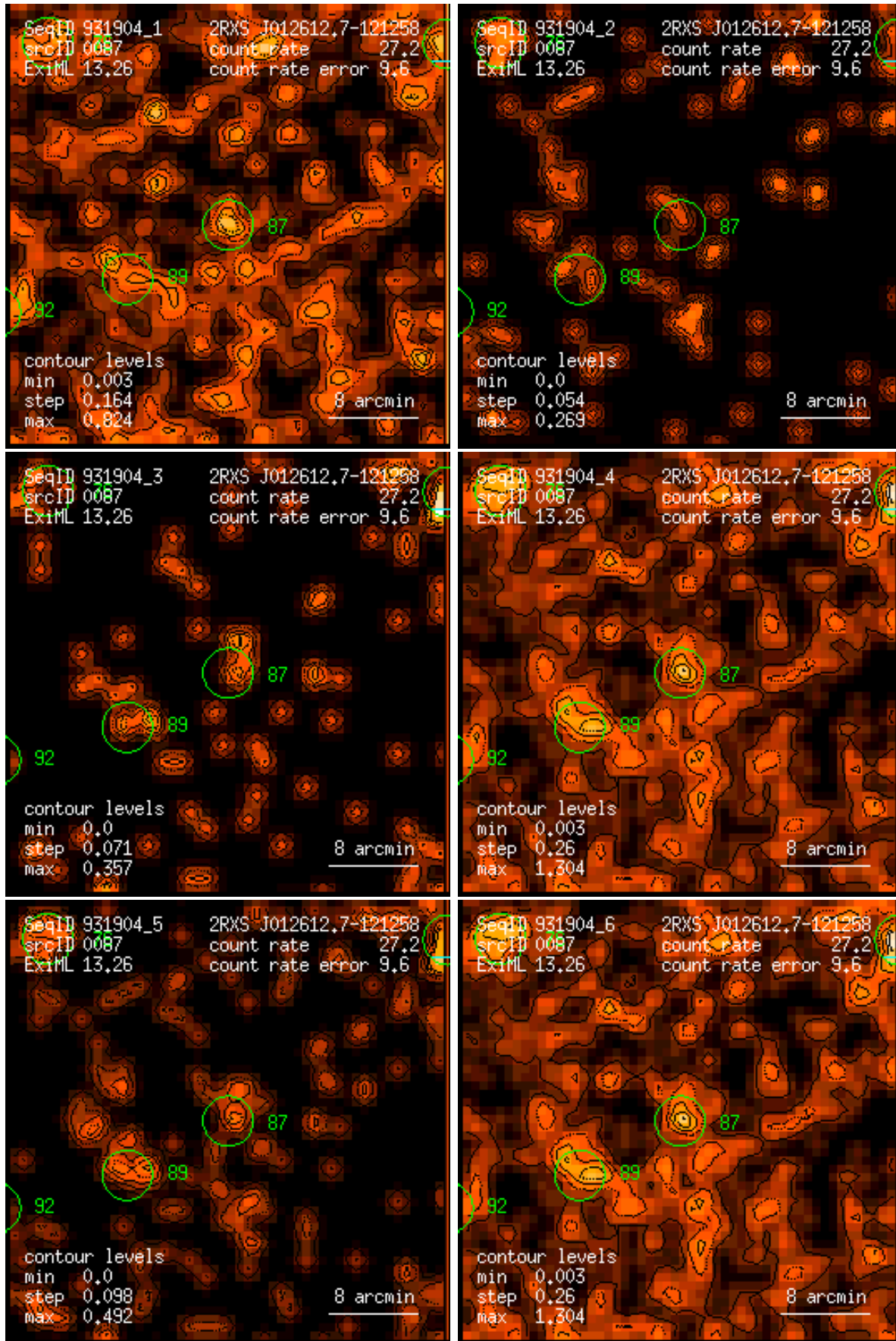
Figure 87: RASS 931904: detection 0087: band rate images, Gaussian filter: (1) PSPC channels 11 – 41, (2) 52 – 90, (3) 91 – 201, (4) 11 – 235, (5) 52 – 201, (6) 11 – 201. Broad band rates in counts/ks. Band rate contour levels in counts/ks/arcmin 2 .
