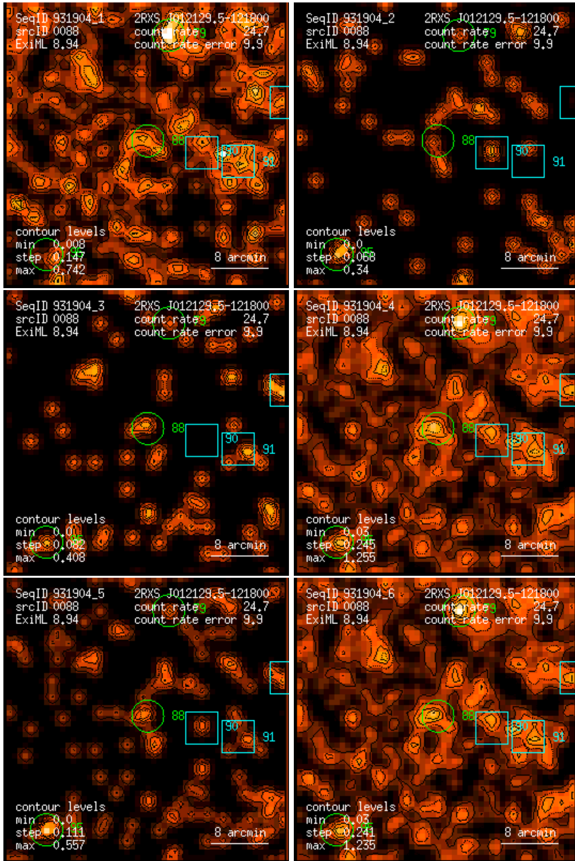
Figure 88: RASS 931904: detection 0088: band rate images, Gaussian filter: (1) PSPC channels 11 – 41, (2) 52 – 90, (3) 91 – 201, (4) 11 – 235, (5) 52 – 201, (6) 11 – 201. Broad band rates in counts/ks. Band rate contour levels in counts/ks/arcmin 2 .
