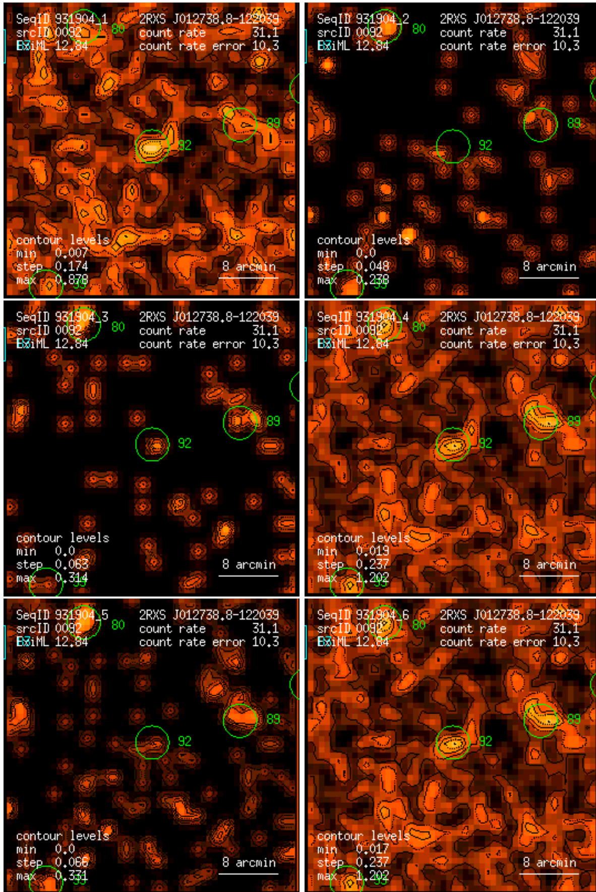
Figure 92: RASS 931904: detection 0092: band rate images, Gaussian filter: (1) PSPC channels 11 – 41, (2) 52 – 90, (3) 91 – 201, (4) 11 – 235, (5) 52 – 201, (6) 11 – 201. Broad band rates in counts/ks. Band rate contour levels in counts/ks/arcmin 2 .
