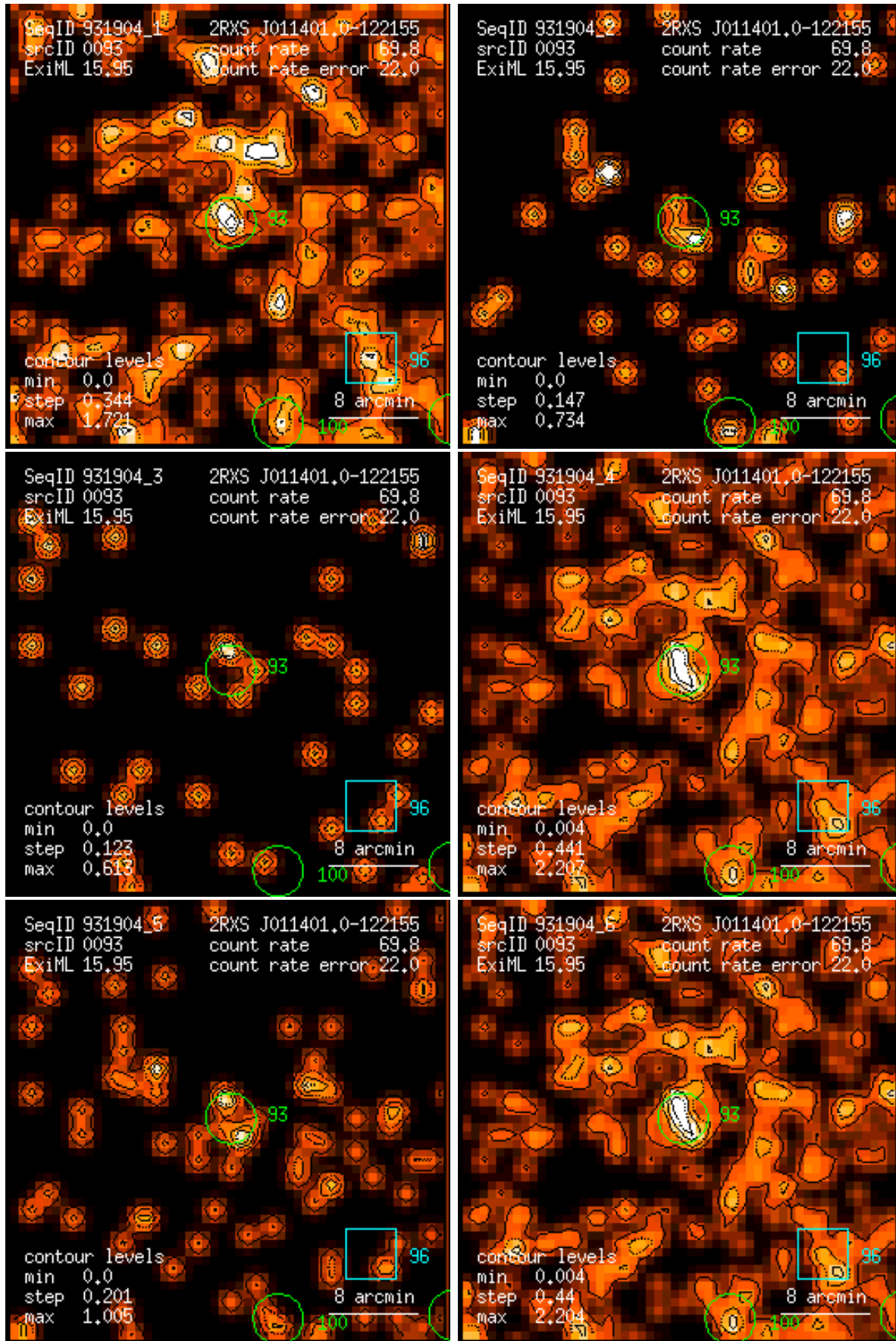
Figure 93: RASS 931904: detection 0093: band rate images, Gaussian filter: (1) PSPC channels 11 – 41, (2) 52 – 90, (3) 91 – 201, (4) 11 – 235, (5) 52 – 201, (6) 11 – 201. Broad band rates in counts/ks. Band rate contour levels in counts/ks/arcmin 2 .
