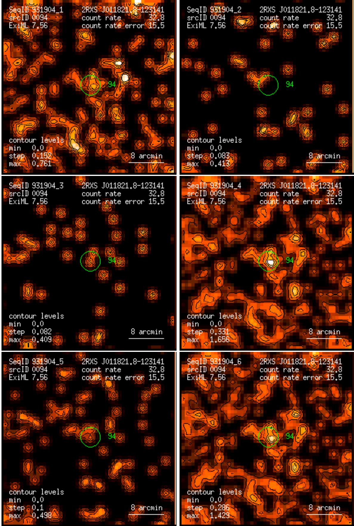
Figure 94: RASS 931904: detection 0094: band rate images, Gaussian filter: (1) PSPC channels 11 – 41, (2) 52 – 90, (3) 91 – 201, (4) 11 – 235, (5) 52 – 201, (6) 11 – 201. Broad band rates in counts/ks. Band rate contour levels in counts/ks/arcmin 2 .
