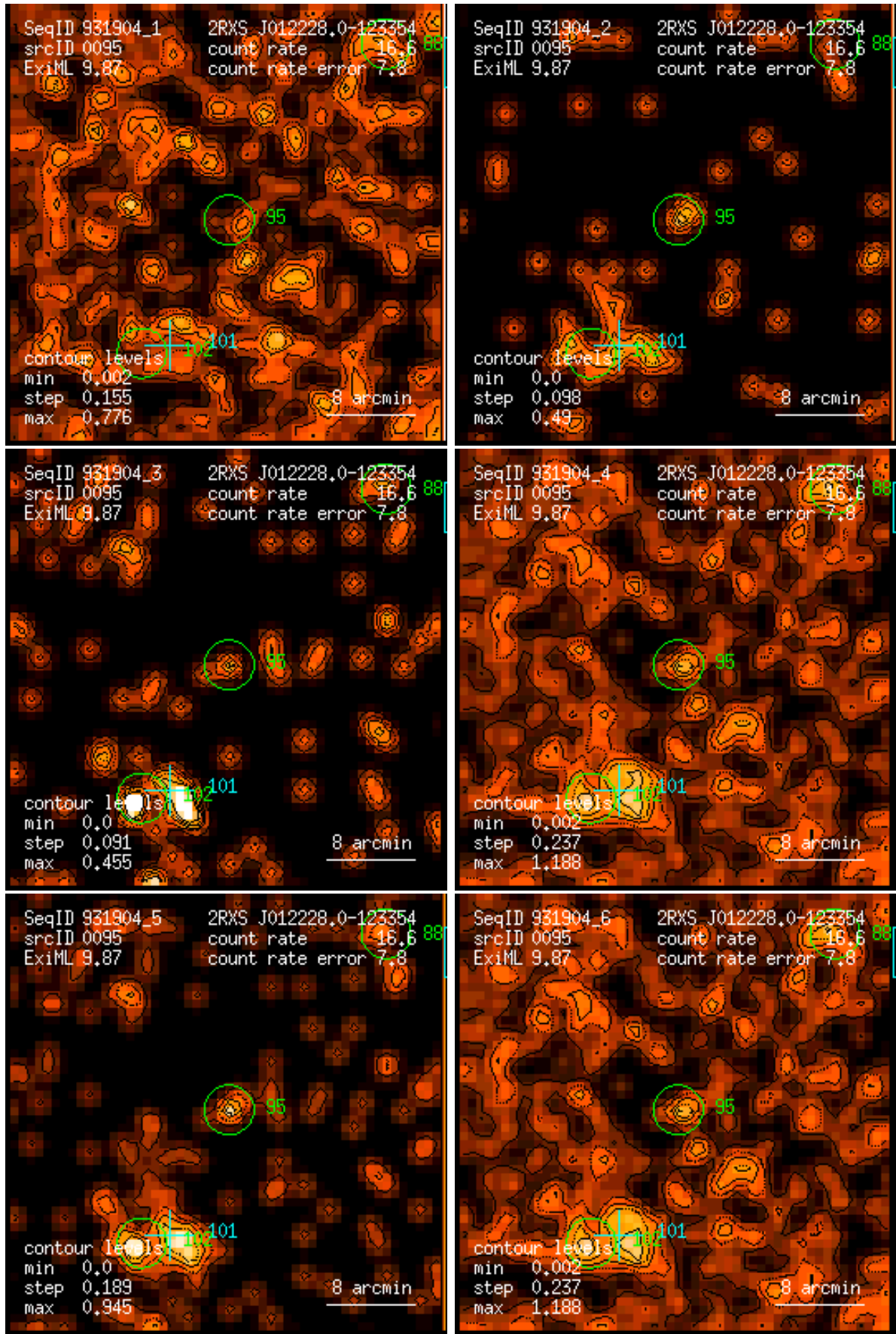
Figure 95: RASS 931904: detection 0095: band rate images, Gaussian filter: (1) PSPC channels 11 – 41, (2) 52 – 90, (3) 91 – 201, (4) 11 – 235, (5) 52 – 201, (6) 11 – 201. Broad band rates in counts/ks. Band rate contour levels in counts/ks/arcmin 2 .
