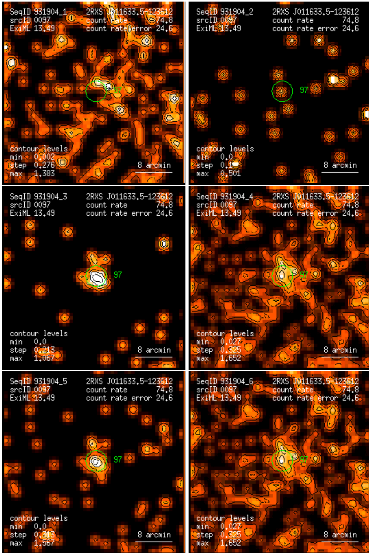
Figure 97: RASS 931904: detection 0097: band rate images, Gaussian filter: (1) PSPC channels 11 – 41, (2) 52 – 90, (3) 91 – 201, (4) 11 – 235, (5) 52 – 201, (6) 11 – 201. Broad band rates in counts/ks. Band rate contour levels in counts/ks/arcmin 2 .
