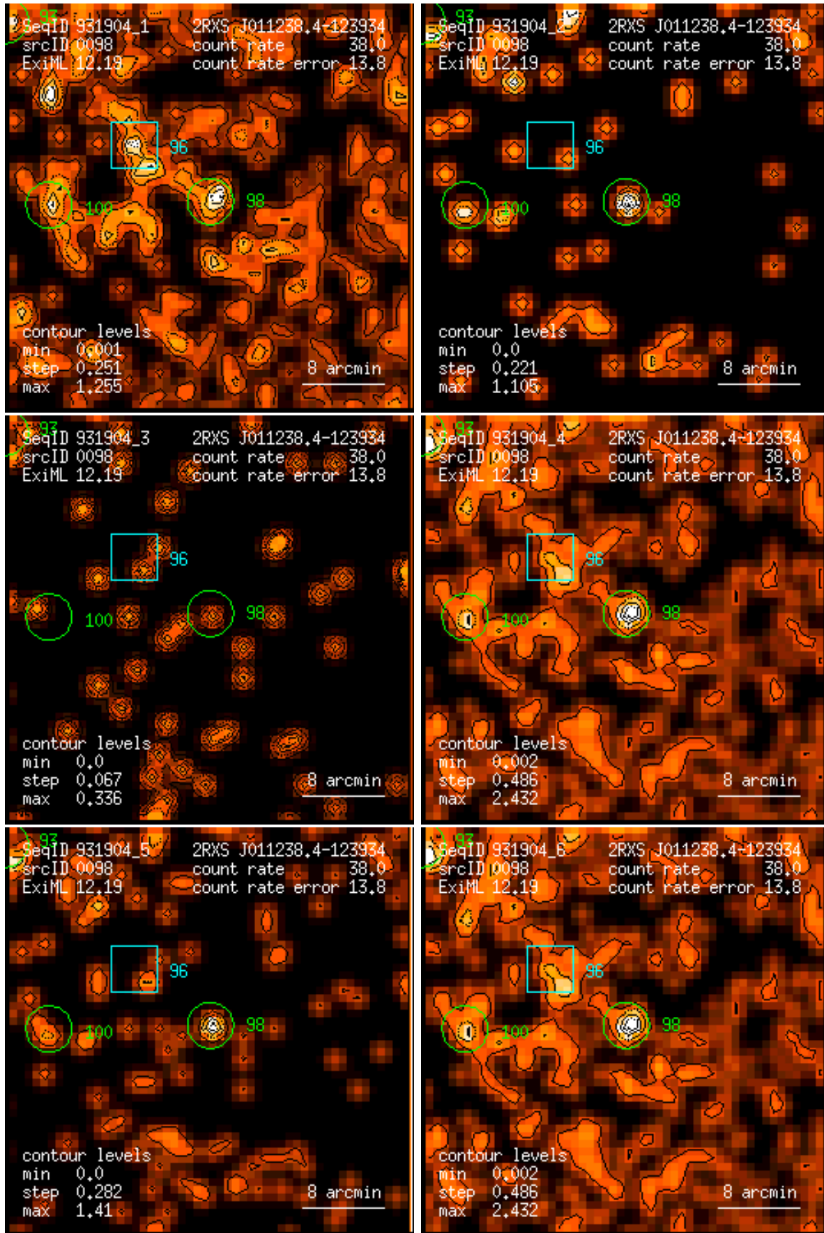
Figure 98: RASS 931904: detection 0098: band rate images, Gaussian filter: (1) PSPC channels 11 – 41, (2) 52 – 90, (3) 91 – 201, (4) 11 – 235, (5) 52 – 201, (6) 11 – 201. Broad band rates in counts/ks. Band rate contour levels in counts/ks/arcmin 2 .
