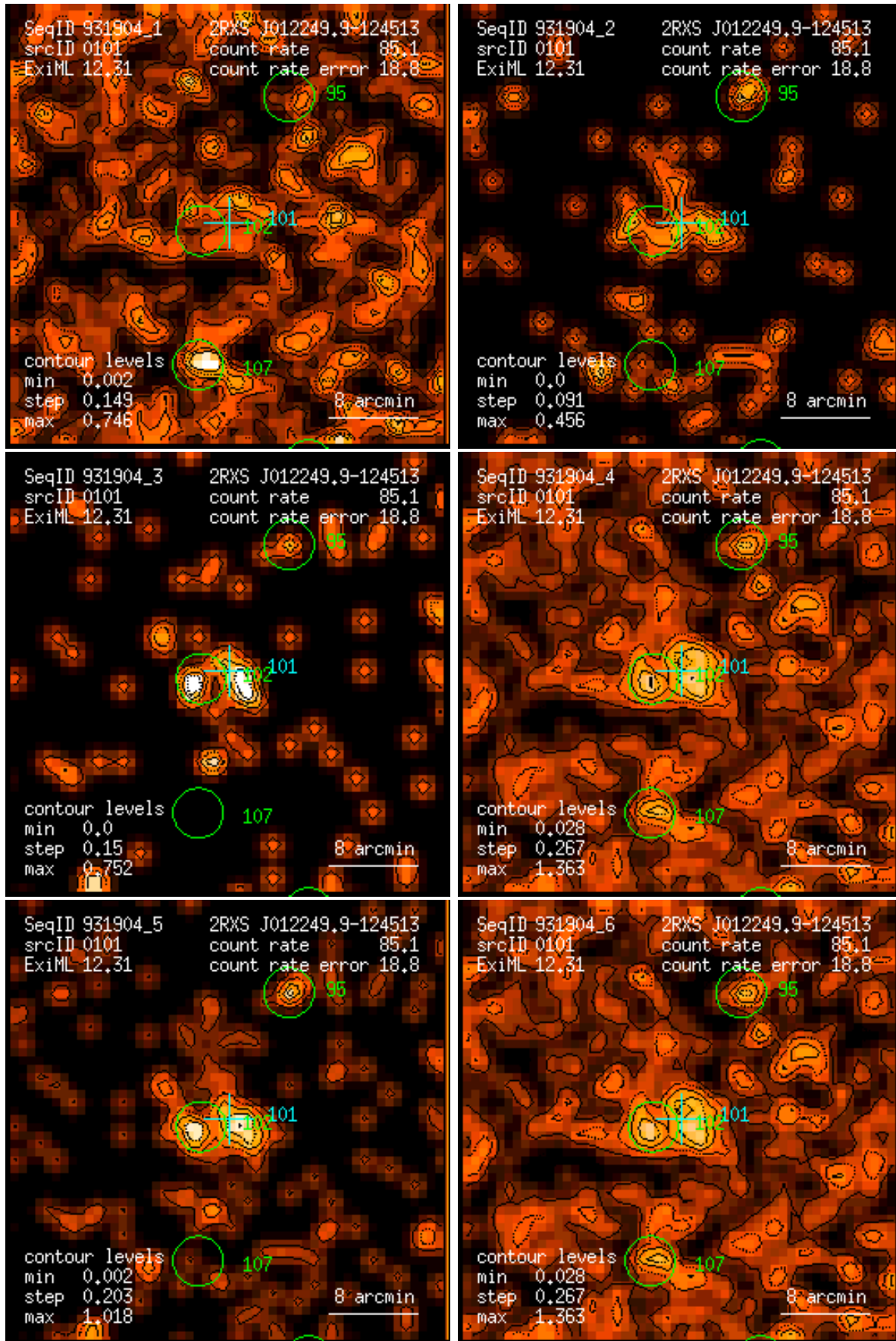
Figure 101: RASS 931904: detection 0101: band rate images, Gaussian filter: (1) PSPC channels 11 – 41, (2) 52 – 90, (3) 91 – 201, (4) 11 – 235, (5) 52 – 201, (6) 11 – 201. Broad band rates in counts/ks. Band rate contour levels in counts/ks/arcmin 2 .
