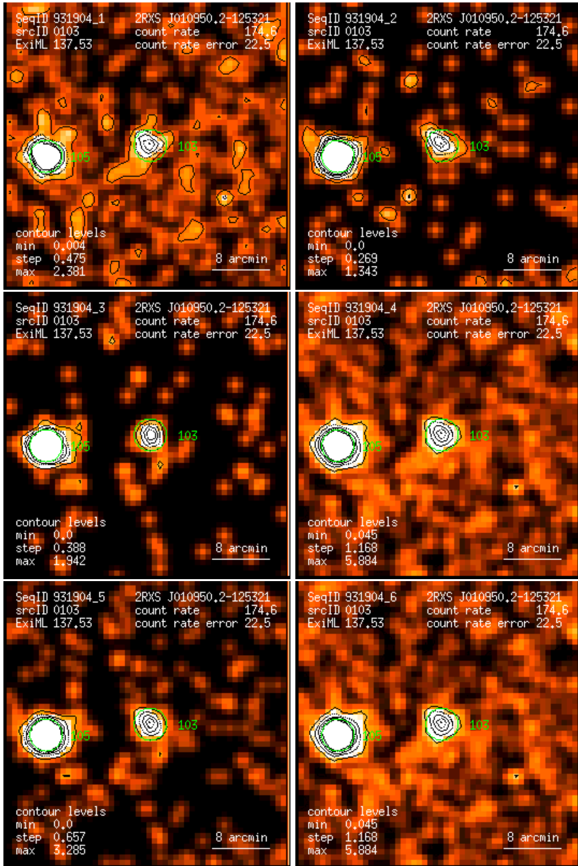
Figure 103: RASS 931904: detection 0103: band rate images, Gaussian filter: (1) PSPC channels 11 – 41, (2) 52 – 90, (3) 91 – 201, (4) 11 – 235, (5) 52 – 201, (6) 11 – 201. Broad band rates in counts/ks. Band rate contour levels in counts/ks/arcmin 2 .
