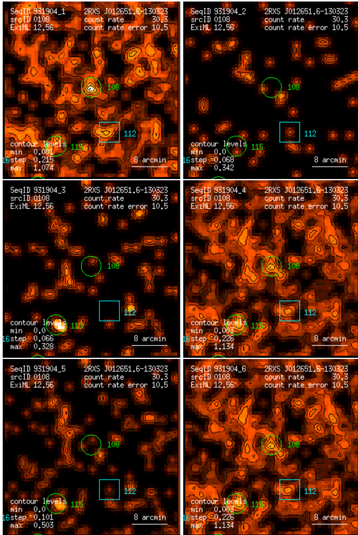
Figure 108: RASS 931904: detection 0108: band rate images, Gaussian filter: (1) PSPC channels 11 – 41, (2) 52 – 90, (3) 91 – 201, (4) 11 – 235, (5) 52 – 201, (6) 11 – 201. Broad band rates in counts/ks. Band rate contour levels in counts/ks/arcmin 2 .
