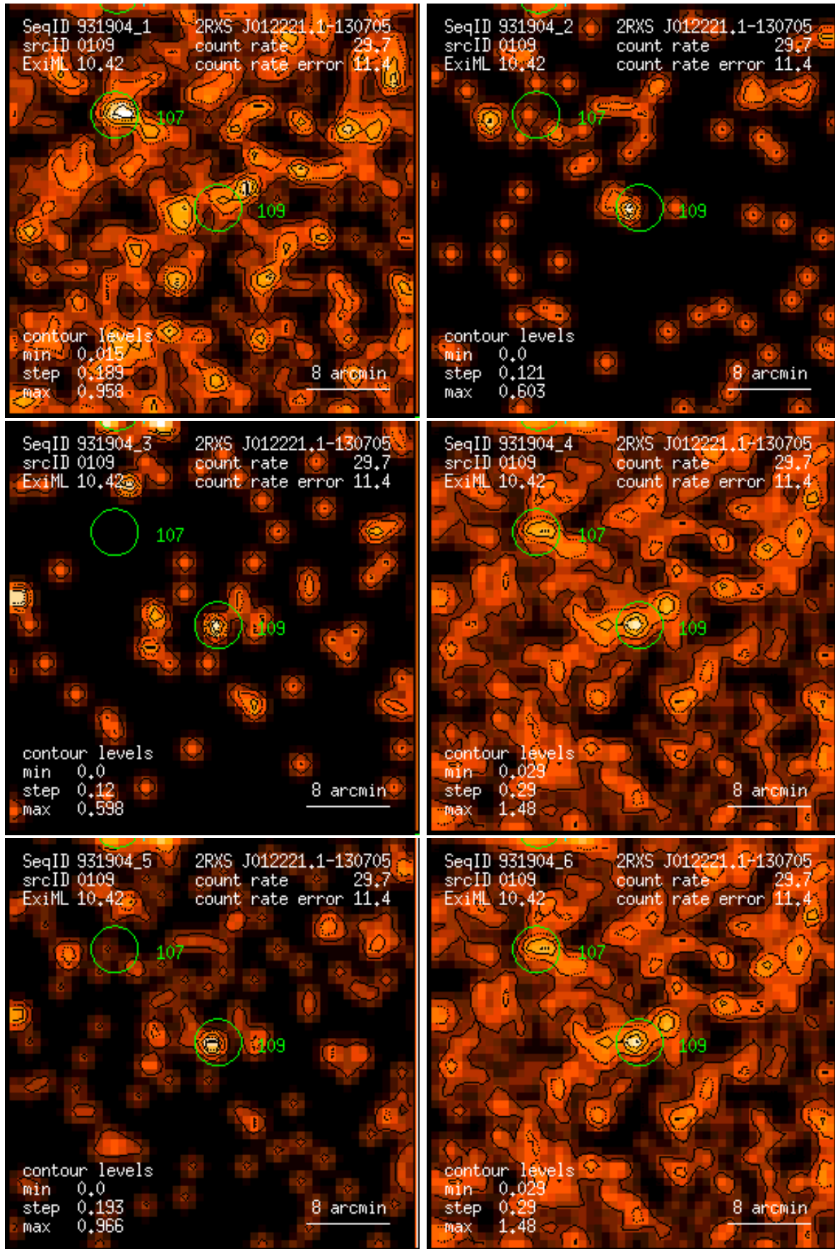
Figure 109: RASS 931904: detection 0109: band rate images, Gaussian filter: (1) PSPC channels 11 – 41, (2) 52 – 90, (3) 91 – 201, (4) 11 – 235, (5) 52 – 201, (6) 11 – 201. Broad band rates in counts/ks. Band rate contour levels in counts/ks/arcmin 2 .
