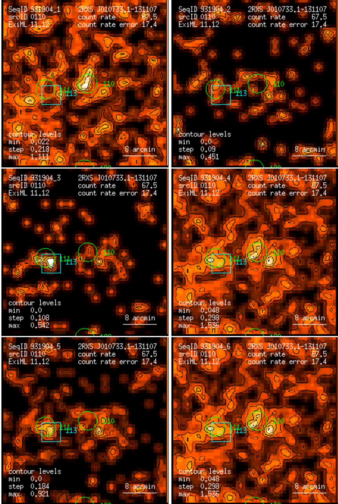
Figure 110: RASS 931904: detection 0110: band rate images, Gaussian filter: (1) PSPC channels 11 – 41, (2) 52 – 90, (3) 91 – 201, (4) 11 – 235, (5) 52 – 201, (6) 11 – 201. Broad band rates in counts/ks. Band rate contour levels in counts/ks/arcmin 2 .
