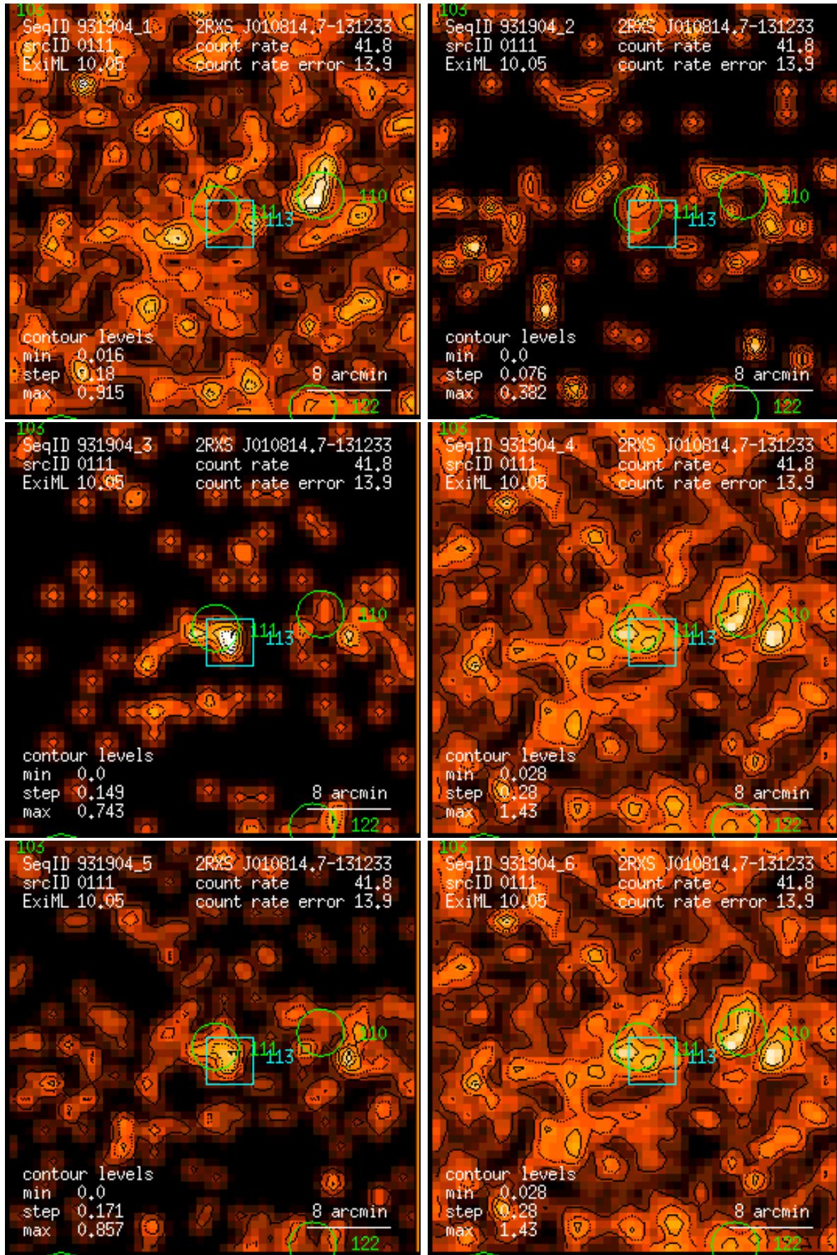
Figure 111: RASS 931904: detection 0111: band rate images, Gaussian filter: (1) PSPC channels 11 – 41, (2) 52 – 90, (3) 91 – 201, (4) 11 – 235, (5) 52 – 201, (6) 11 – 201. Broad band rates in counts/ks. Band rate contour levels in counts/ks/arcmin 2 .
