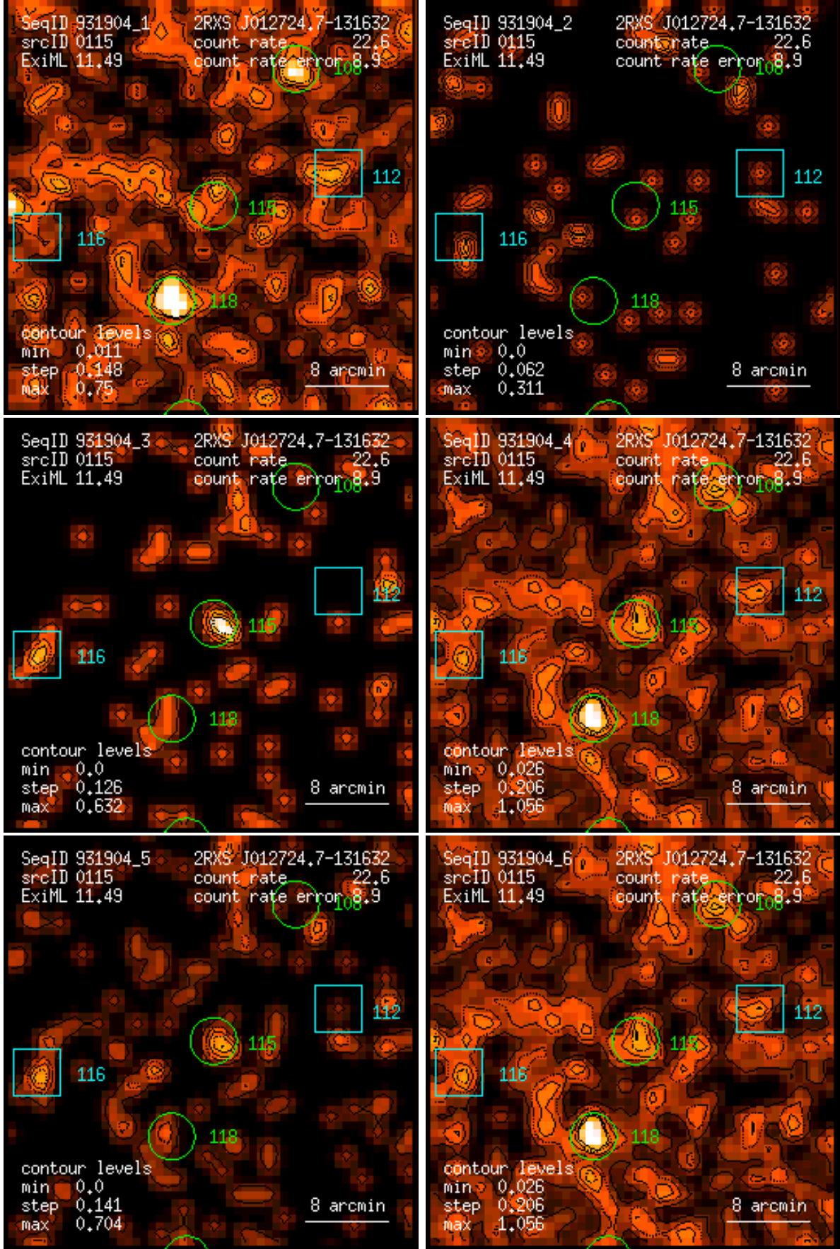
Figure 115: RASS 931904: detection 0115: band rate images, Gaussian filter: (1) PSPC channels 11 – 41, (2) 52 – 90, (3) 91 – 201, (4) 11 – 235, (5) 52 – 201, (6) 11 – 201. Broad band rates in counts/ks. Band rate contour levels in counts/ks/arcmin 2 .
