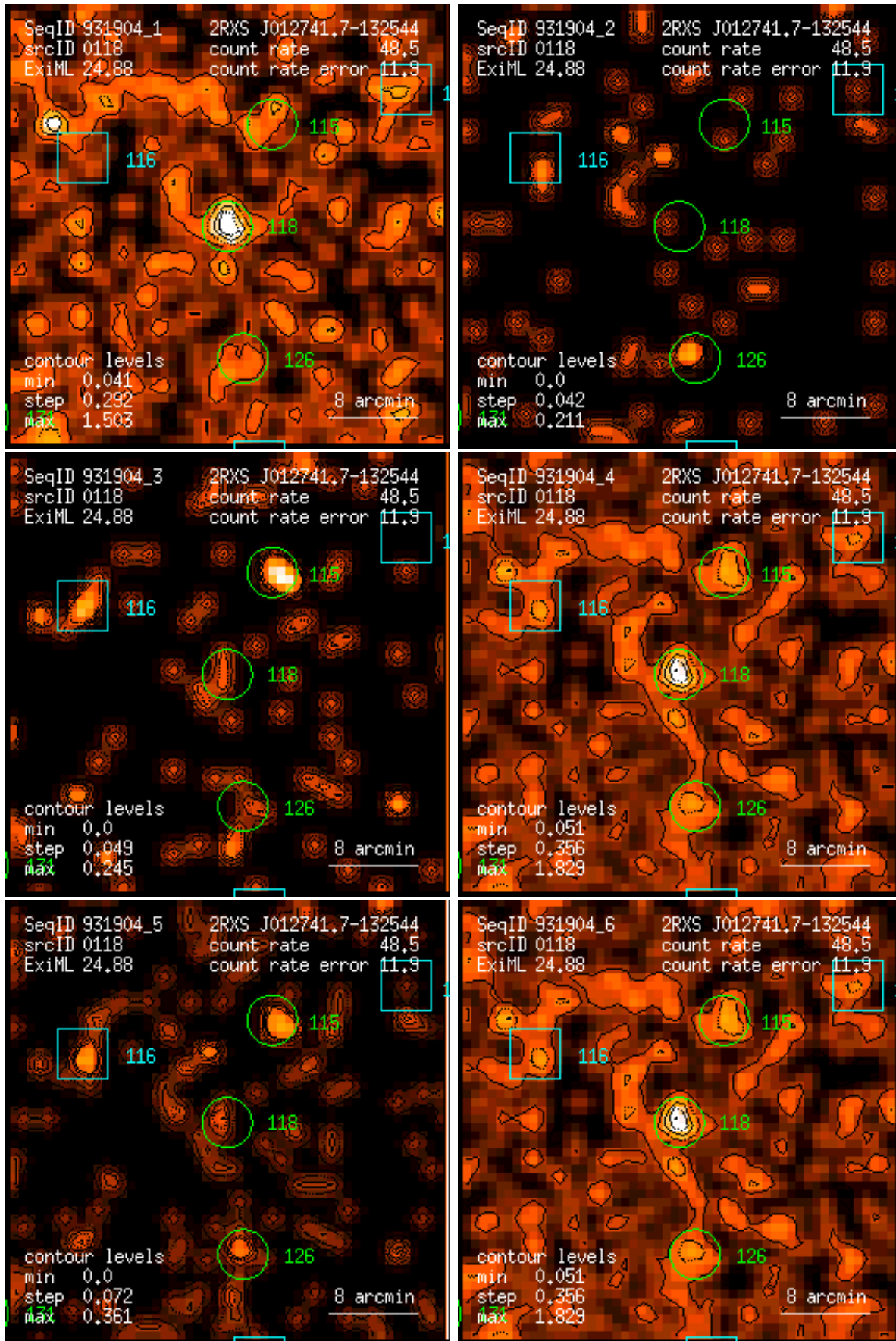
Figure 118: RASS 931904: detection 0118: band rate images, Gaussian filter: (1) PSPPC channels 11 – 41, (2) 52 – 90, (3) 91 – 201, (4) 11 – 235, (5) 52 – 201, (6) 11 – 201. Broad band rates in counts/ks. Band rate contour levels in counts/ks/arcmin 2 .
