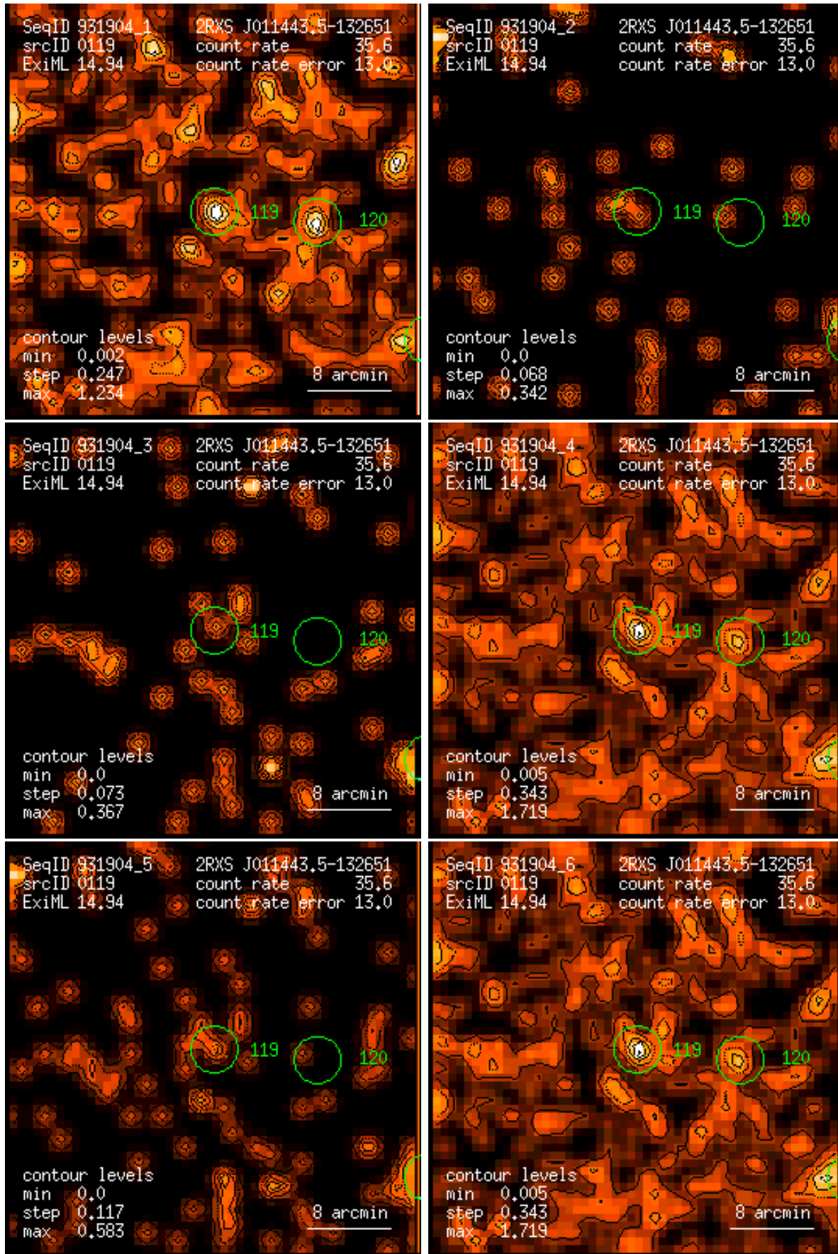
Figure 119: RASS 931904: detection 0119: band rate images, Gaussian filter: (1) PSPC channels 11 – 41, (2) 52 – 90, (3) 91 – 201, (4) 11 – 235, (5) 52 – 201, (6) 11 – 201. Broad band rates in counts/ks. Band rate contour levels in counts/ks/arcmin 2 .
