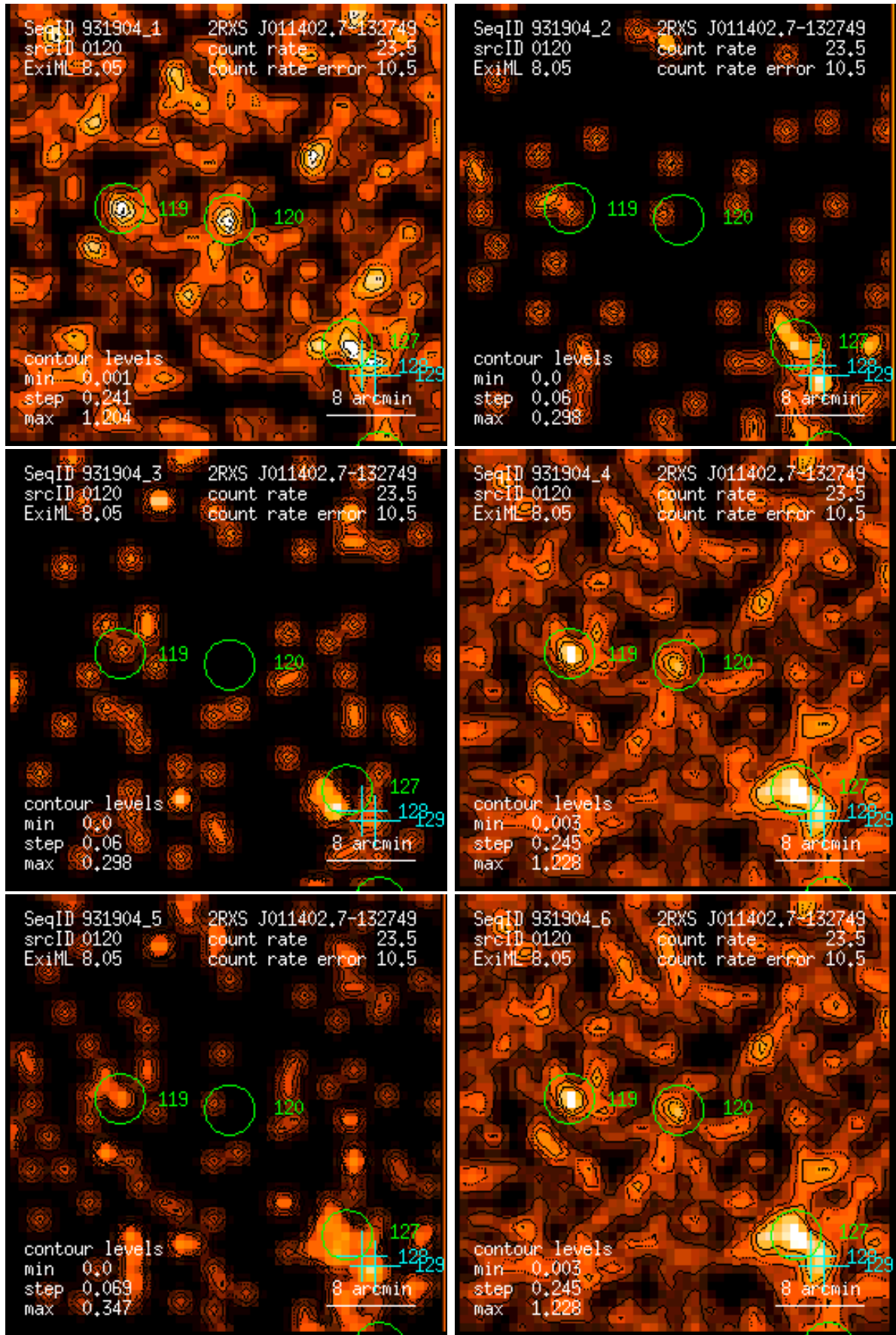
Figure 120: RASS 931904: detection 0120: band rate images, Gaussian filter: (1) PSPC channels 11 – 41, (2) 52 – 90, (3) 91 – 201, (4) 11 – 235, (5) 52 – 201, (6) 11 – 201. Broad band rates in counts/ks. Band rate contour levels in counts/ks/arcmin 2 .
