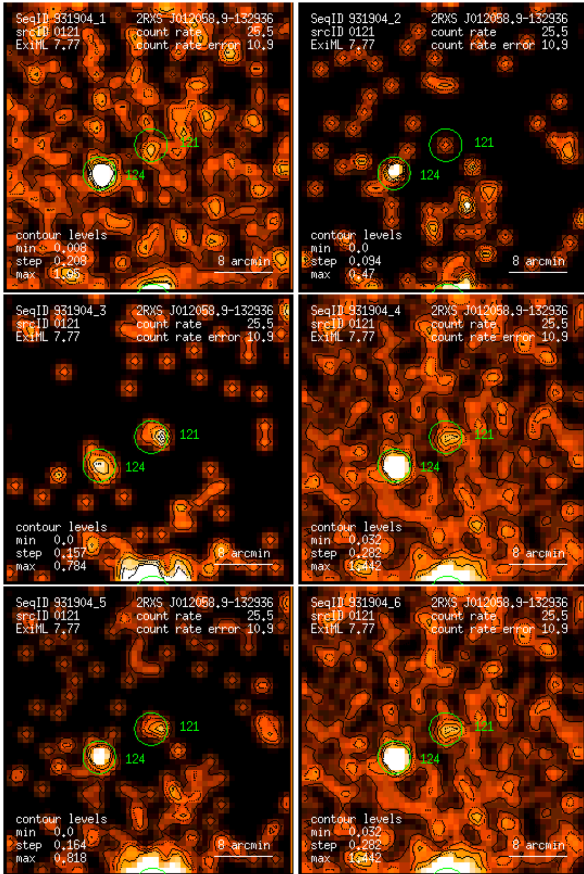
Figure 121: RASS 931904: detection 0121: band rate images, Gaussian filter: (1) PSPC channels 11 – 41, (2) 52 – 90, (3) 91 – 201, (4) 11 – 235, (5) 52 – 201, (6) 11 – 201. Broad band rates in counts/ks. Band rate contour levels in counts/ks/arcmin 2 .
