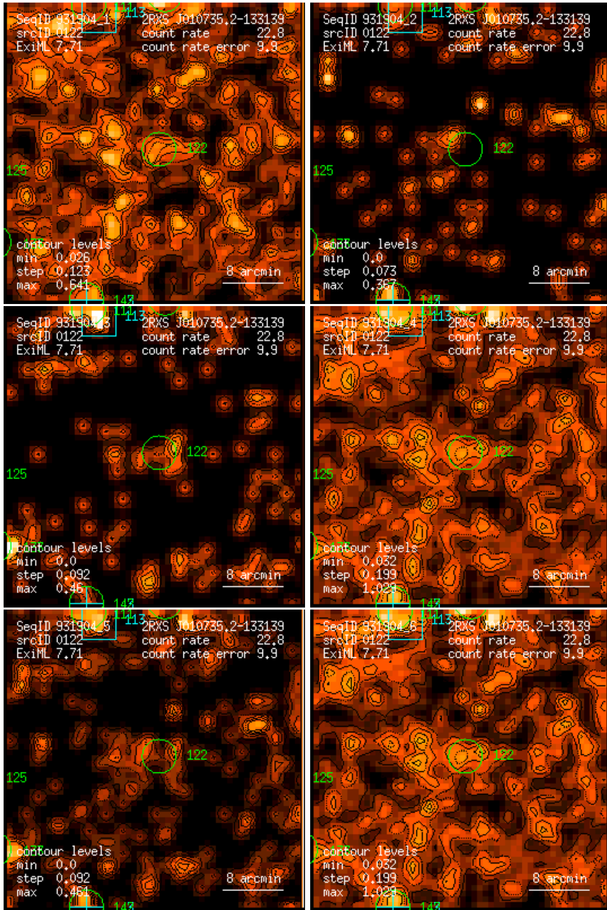
Figure 122: RASS 931904: detection 0122: band rate images, Gaussian filter: (1) PSPC channels 11 – 41, (2) 52 – 90, (3) 91 – 201, (4) 11 – 235, (5) 52 – 201, (6) 11 – 201. Broad band rates in counts/ks. Band rate contour levels in counts/ks/arcmin 2 .
