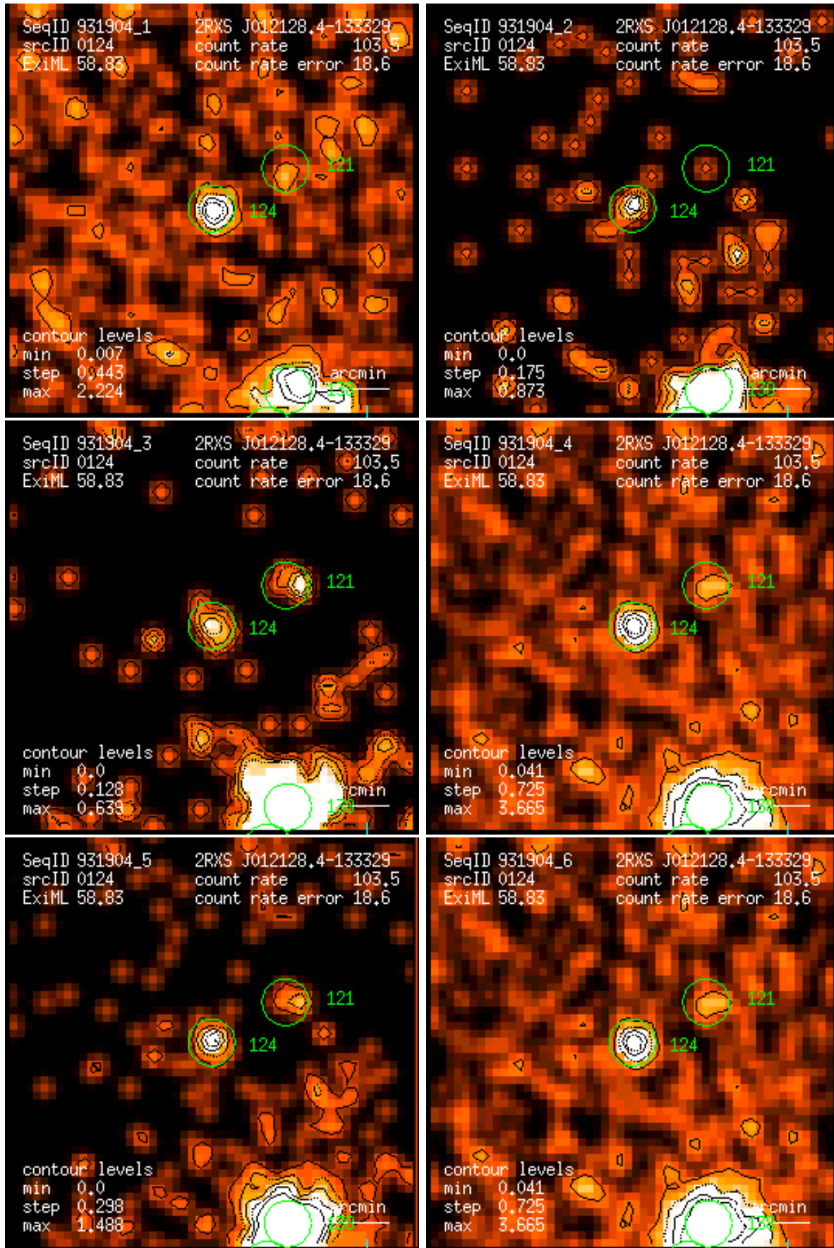
Figure 124: RASS 931904: detection 0124: band rate images, Gaussian filter: (1) PSPC channels 11 – 41, (2) 52 – 90, (3) 91 – 201, (4) 11 – 235, (5) 52 – 201, (6) 11 – 201. Broad band rates in counts/ks. Band rate contour levels in counts/ks/arcmin 2 .
