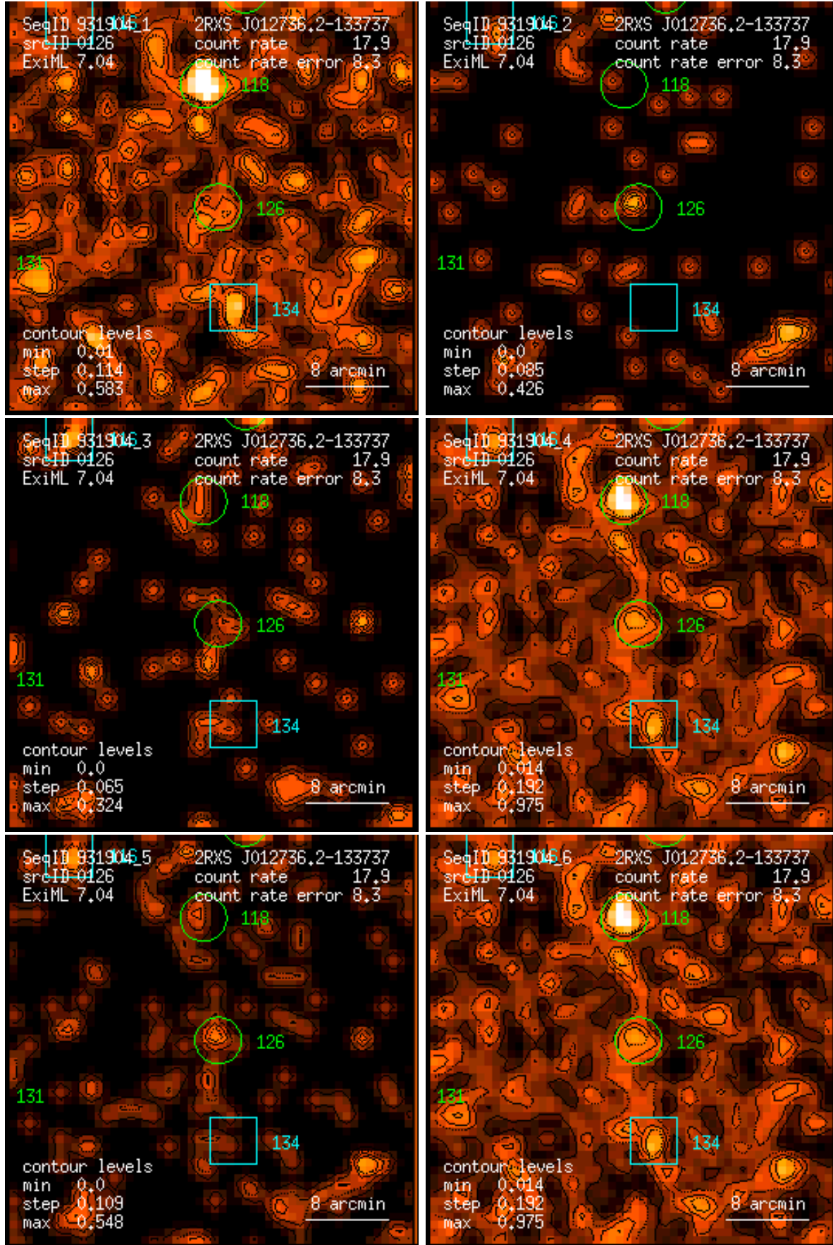
Figure 126: RASS 931904: detection 0126: band rate images, Gaussian filter: (1) PSPC channels 11 – 41, (2) 52 – 90, (3) 91 – 201, (4) 11 – 235, (5) 52 – 201, (6) 11 – 201. Broad band rates in counts/ks. Band rate contour levels in counts/ks/arcmin 2 .
